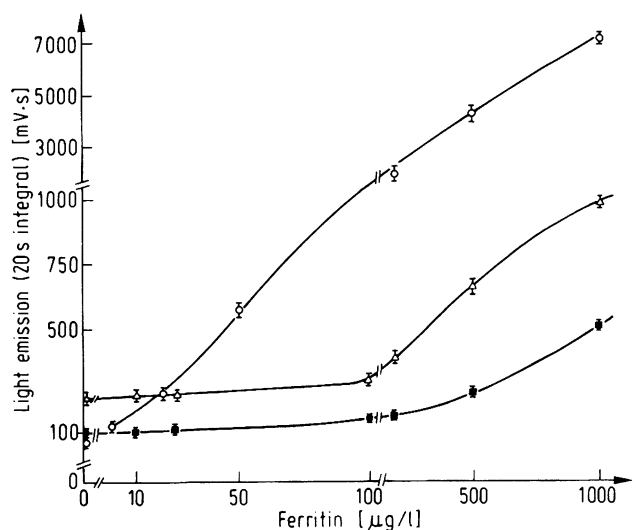
Fig. 2. Comparison of three ferritin assays using diazoluminol (△—△ ILSA; ■—■ ILMA) and N-(4-aminobutyl)-N-ethyl isoluminol hemisuccinamide (○—○ ILMA) labelled antibodies. Please note that the scales are not linear. The symbols and their significance are as in figure 1.
