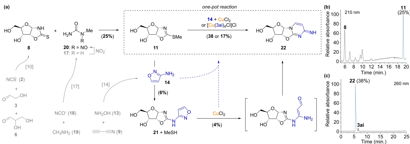
Figure 2. a) Reaction sequence that generates precursor molecules of cytidine upon merging of the Sutherland-Powner and Carell pathways; HPLC chromatogram for (b) the methylation of ribo-2-thiooxazoline 8 to ribo-2-(methylthio)oxazoline 11 and (c) its conversion to ribo-anhydrocytidine 22.
