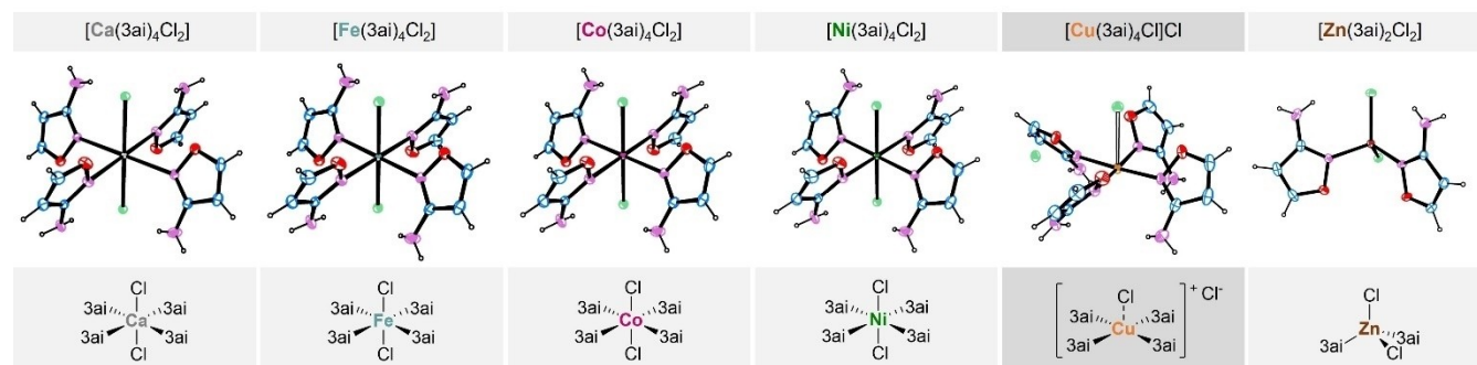
Figure 3. Crystal structures of 3-aminoisoxazole (3ai, 14 ) complexes with various \text{M}^{2+} ions. In an experiment with a mixture of \text{M}^{2+} salts, the \text{Cu}^{2+} complex precipitates first. [21]
