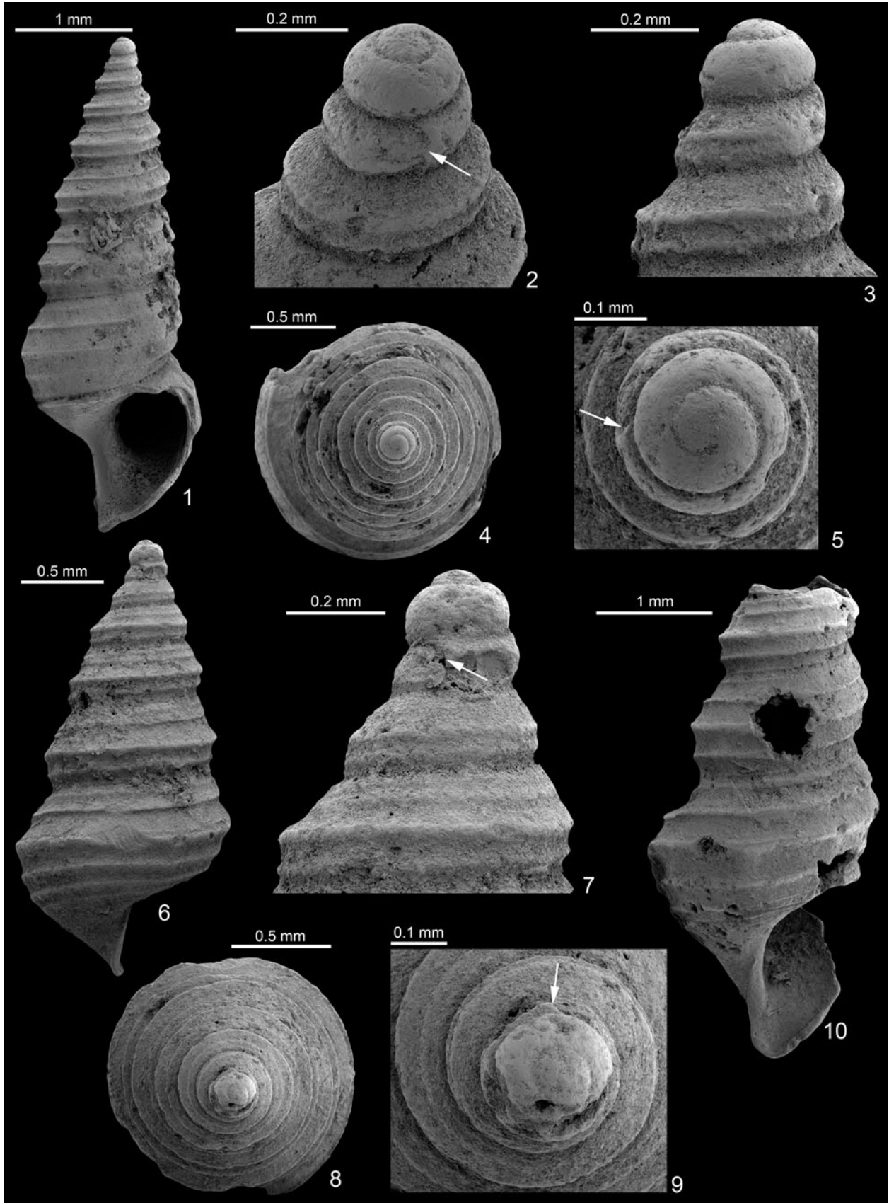
Figure 13. Stegocoelia (Hypergonia) variabilis (Donald, 1895), Law [Quarry], Dalry, Ayrshire, Scotland; Lower Limestone Group (Viséan). (1–5) NHMUK PI PG 10265. (6–9) NHMUK PI PG 10266. (10) NHMUK PI PG 10267. Arrows = protoconch-teleoconch boundary.
