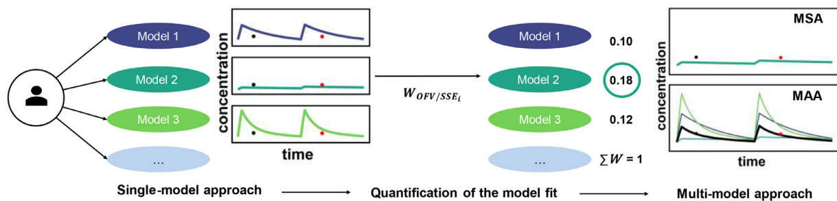
Fig. 1. Workflow from single-model approach to a multi-model approach. Single-model approach: Estimation of PopPK-model profiles for each patient using Bayesian forecasting from first TDM-sample (= black point) to future TDM-samples (= red point), each model is evaluated separately. Quantification of the model fit: For each patient the fractional individual weight of the model fit based on the first sample is calculated using a predefined weighting scheme (e.g., W_{OFV} or SSE ). Multi-model approach: The algorithm (i) either selects the best fitting model for each patient (= maximum W_{OFV/SSE} ) → model selection algorithm (MSA) or (ii) calculates a new prediction based on the individual weights of the models = \sum_1^n (W_{OFV, SSE} \cdot c_{pred}) → model averaging algorithm (MAA). PopPK: Population pharmacokinetic; W: calculated fractional weight; SSE: sum of squares error; OFV: objective function value; c: concentration; pred: predicted; n: set of models; i: individual patient; TDM: therapeutic drug monitoring.
