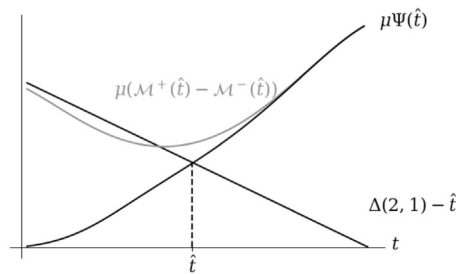
Fig. 2. Equilibrium for K = 2 .
