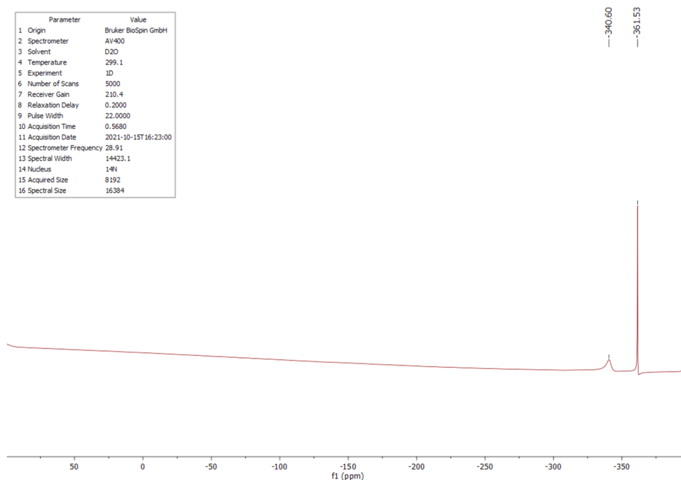
Figure 8 The ^{14}\text{N} NMR spectrum of (I) in \text{D}_2\text{O} .
