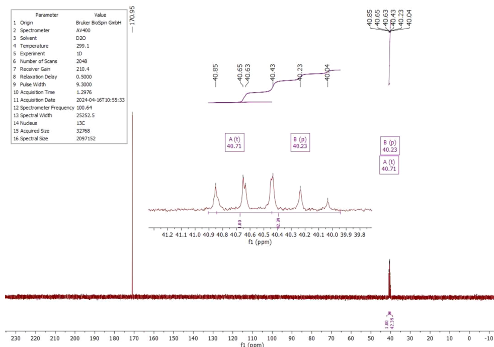
Figure 7 The ^{13}\text{C} NMR spectrum of malonic acid ( \text{C}_3\text{H}_4\text{O}_4 ) in \text{D}_2\text{O} .
