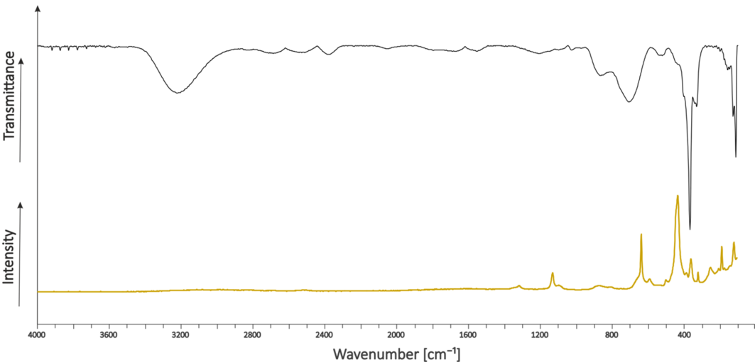
Figure 2 Vibrational spectra of Na[GeF 5 ] 2 ·2HF, showing IR (top) and Raman (bottom).
