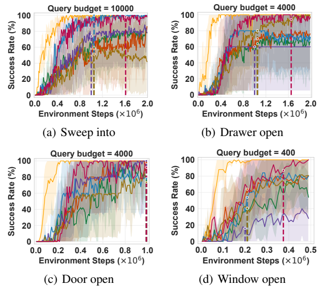
Figure 3: Learning curves on manipulation tasks as measured on the success rate. The solid line and shaded regions represent the mean and standard deviation, respectively, across five runs. The vertical dashed lines indicate the end of the querying process.
