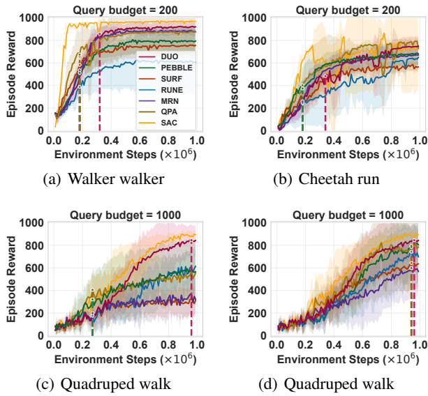
Figure 2: Learning curves on locomotion tasks as measured on the ground truth reward. The solid line and shaded regions represent the mean and standard deviation, respectively, across five runs. The vertical dashed lines indicate the end of the querying process.
