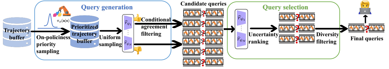
Figure 1: DUO consists of two main phases: query generation and query selection. Generation starts from the buffer of the agent’s trajectories. A subset of trajectories is sampled with priority regarding on-policiness under the current policy. We then perform random segmenting and pairing, followed by filtering based on whether or not the decision boundary is included in the ensemble’s predictions. The selection from the resulting candidate queries is based on the estimated epistemic uncertainty of the preference predictions and is further filtered by diversity using k-means clustering.
