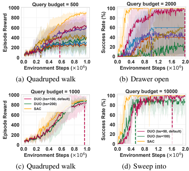
Figure 4: Sensitivity study on different tasks. Figs. 4(a) and 4(b) show results of different query budget, and Figs. 4(c) and 4(d) show results of different predefined query batch size.
