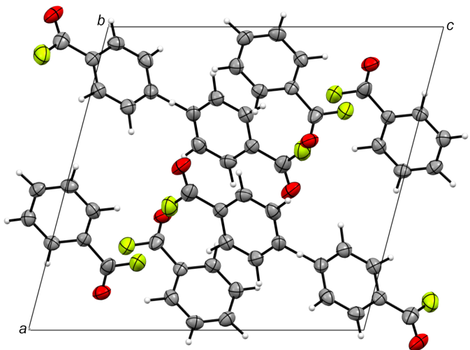
Figure 2 Crystal structure of benzoyl fluoride ( 1 ), viewed along the b axis. Displacement ellipsoids are drawn at the 50% probability level.
