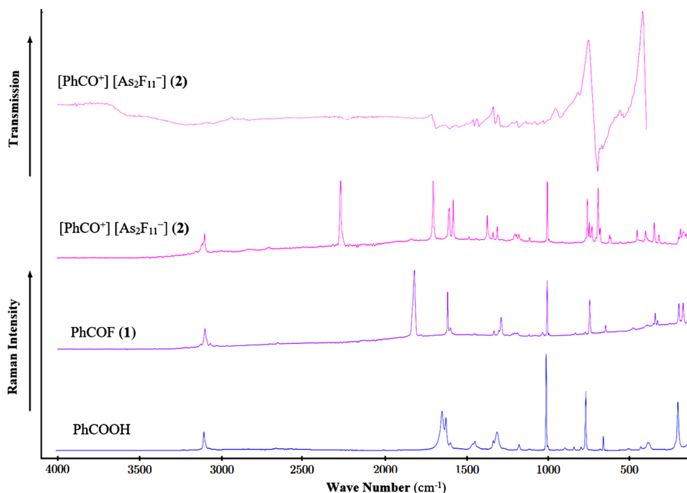
Figure 1 IR and Raman spectra of PhCOOH, PhCOF ( 1 ) and benzoacyl cation undecafluorodiarsonate ( 2 ).
