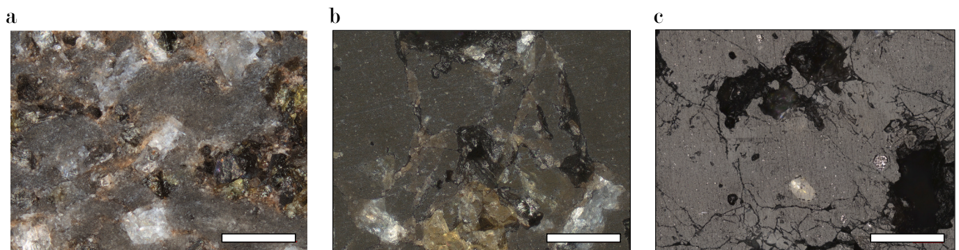
Fig. 5. Post-experimental sample textures in (a–b) plane light and (c) reflected light (captured using a Keyence VK-X 1000 scanning microscope). (a) A sample that was deformed during ‘slow’ deformation (see text). (b) and (c) samples deformed during ‘fast deformation’ (see text). All scale bars are 500 \mu\text{m} .
