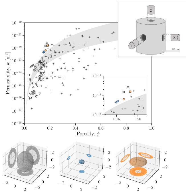
Fig. 6. The permeability of our samples before and after high-temperature deformation to low ( \varepsilon = 0.2 ) axial strain. Here we show the pre-experimental sample in grey, the post experimental sample for the ‘slow experiment’ in blue, and the post experimental sample for the ‘fast experiment’ in orange (as in Fig. 2). The circles represent the permeability in the axial direction (z), and the squares represent the mean of the permeability in the two radial directions (y and x; the range between the two values is smaller than the point). We also show the results of the 24 smaller samples where the post-experiment permeabilities could only be measured in the axial direction (unfilled circles). Uncertainties on the permeability and porosity determinations are smaller than the data points shown. We also show the compiled suite of volcanic rock permeabilities for the products of effusive eruptions (crosses; Colombier et al., 2017) and the proposed k(\phi) empirical laws (Mueller et al., 2005) of the form k = k_0 \phi^n with k_0 = 1 \times 10^{-17} \text{ m}^2 bounded by n = 3 and n = 3.8 (these two empirical laws are given by the upper and lower bounds on the grey area). For instructive comparison, we also give data for banded Colima dome rocks that show significant anisotropy between the band-parallel direction (upward triangles) and band-perpendicular direction (downward triangles; Farquharson et al., 2016). Inset: a zoom-in on the data in the main plot. Below we show anisotropy ellipsoids where the axes values are given in darcy, rather than \text{m}^2 , simply for clarity (1 darcy is approximately 1 \times 10^{-12} \text{ m}^2 ). These ellipsoids are designed to be illustrative of the degree of anisotropy, such that the relative shape change is of particular interest. (For interpretation of the references to colour in this figure legend, the reader is referred to the web version of this article.)
