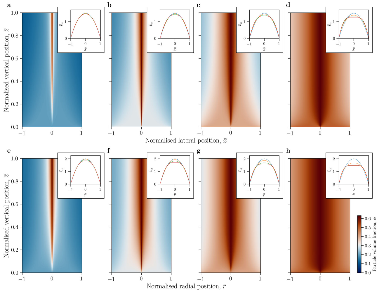
Fig. 2 | Normalised conduit model outputs for shear-induced crystal migration and the development of plug flow. a–d The result for flow in a dyke geometry. e–h The result for flow in a cylindrical conduit. The inlet crystal volume fraction is homogeneous at \bar{z} = 0 and is set to \phi_0 = 0.2 in (a, e) \phi_0 = 0.3 in (b, f) \phi_0 = 0.4 in (c, g) and \phi_0 = 0.5 in (d, h). Insets: The radial distribution of vertical mixture
