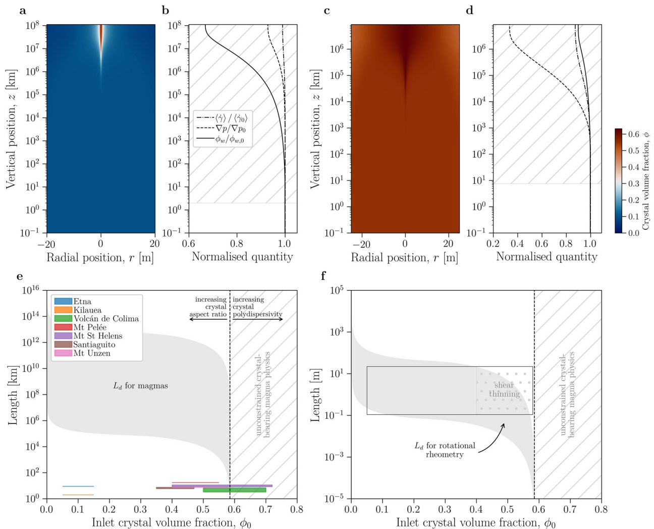
Fig. 3 | Applications of the conduit flow model (Fig. 2) to volcanic and experimental scenarios. a, b The result of an application to a typical basaltic conduit using inputs for Kilauea volcano (USA) of \phi_0 = 0.1 , a = 600 \mu\text{m} , R = 20 \text{ m} , and L_f = 2 \text{ km} , where a shows the dimensional up-conduit development of \phi (as per Fig. 2) and b shows the up-conduit development of the values of the crystal volume fraction at the wall \phi_w , the mixture pressure gradient \nabla p , and the gap-averaged strain rate \langle \dot{\gamma} \rangle , all normalised to the inlet values of those metrics. c, d The same as in (a, b) but for a typical case of a silicic conduit, here using input values for Mt Unzen (Japan) of \phi_0 = 0.55 , a = 300 \mu\text{m} , R = 25 \text{ m} , and L_f = 7.5 \text{ km} . In (b, d) , we use hatching to show the region of the system greater than L_f , which is, therefore, inaccessible; this implies that shear-induced migration is unlikely in both scenarios. e A compilation
