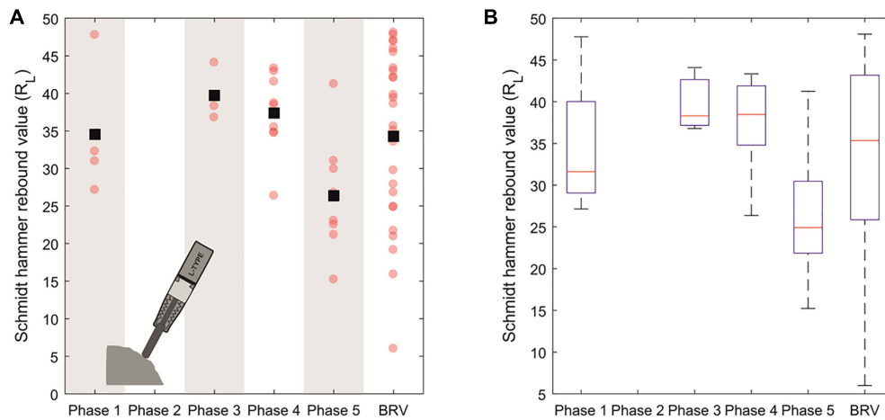
FIGURE 5 | (A) Schmidt hammer rebound value ( R_L ) results from field testing at sampling locations for Phases 1, 3, 4, and 5. Belham River Valley (BRV) results show values obtained on a random selection of blocks from Phases 3, 4, and 5. Raw data shown by circles, with the mean R_L for each phase shown by a square; (B) box plot diagram to show median (red line), mean (black squares), 25th and 75th percentiles, and range for Schmidt hammer rebound values from each phase. Results from BRV span the overall range in values seen in other phases and highlight that Phase 5 material is the weakest of the erupted products tested, although the maximum R_L across all phases is similar.
