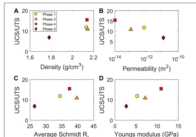
FIGURE 10 | (A) UCS/UTS ratio as a function of density; (B) UCS/UTS ratio as a function of permeability; (C) UCS/UTS ratio as a function of average Schmidt hammer rebound value ( R_L ); and (D) UCS/UTS ratio as a function of Young's modulus. Phase averages shown in each case. A higher UCS/UTS ratio correlates to lower permeabilities, higher Schmidt hammer rebound values, and higher Young's modulus values.
