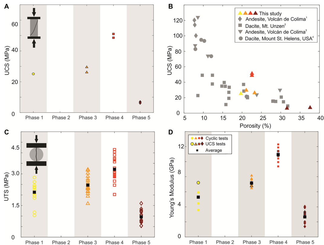
FIGURE 8 | (A) UCS results. UCS is highest in Phase 4, and lowest in Phase 5, while Phases 1 and 3 are intermediate. (B) UCS as a function of porosity, compared with published datasets from other dome-building volcanoes: 1 Heap et al., 2018a (diamonds); 2 Coats et al., 2018 (squares); 3 Heap et al., 2014a (downward triangles); 4 Kendrick et al., 2013 (circles); (C) Tensile strength determined by Brazilian disk testing for samples from eruptive Phases 1, 3, 4, and 5. Each measurement is shown by the hollow markers, with mean tensile strength for each eruptive Phase shown by the black squares. (D) Young's modulus ( E ) determined from both UCS and cyclic tests performed on 26 mm diameter cores and shown by Phase with averages shown for each Phase (black squares). Young's modulus is determined using stress/strain between 40 and 50% of the UCS strength value, from the linear portion of stress/strain curve where we assume elastic behavior.
