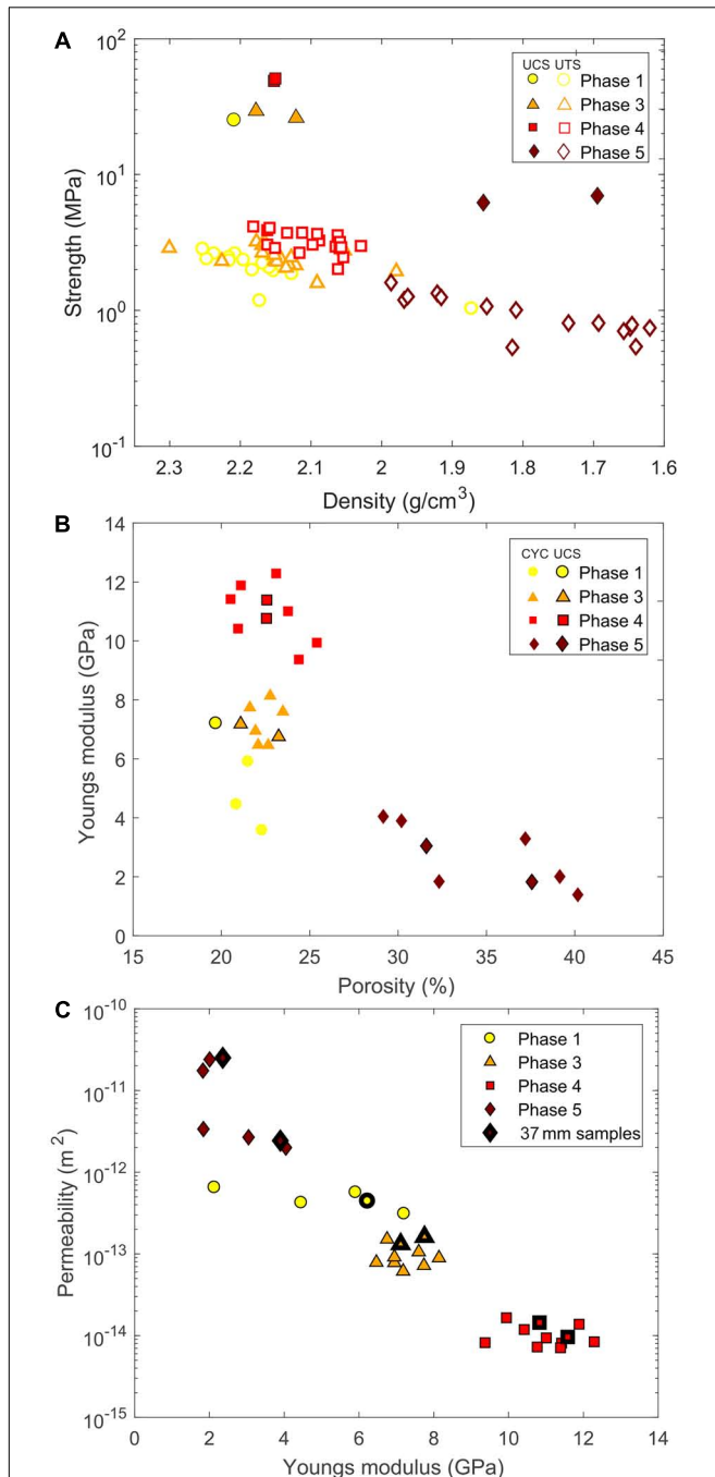
FIGURE 9 | (A) Uniaxial tensile strength (UTS; hollow symbols) and uniaxial compressive strength (UCS; filled symbols) as a function of rock density (a proxy for porosity, see Supplementary Table S1 and Supplementary Figure S1 ). (B) Young's modulus as a function of connected porosity, determined from UCS tests (black symbol outlines) and from cyclic tests (no symbol outline). (C) Permeability as a function of Young's modulus, for 26 mm samples (thin symbol outline) and 37 mm samples (thick symbol outline).
