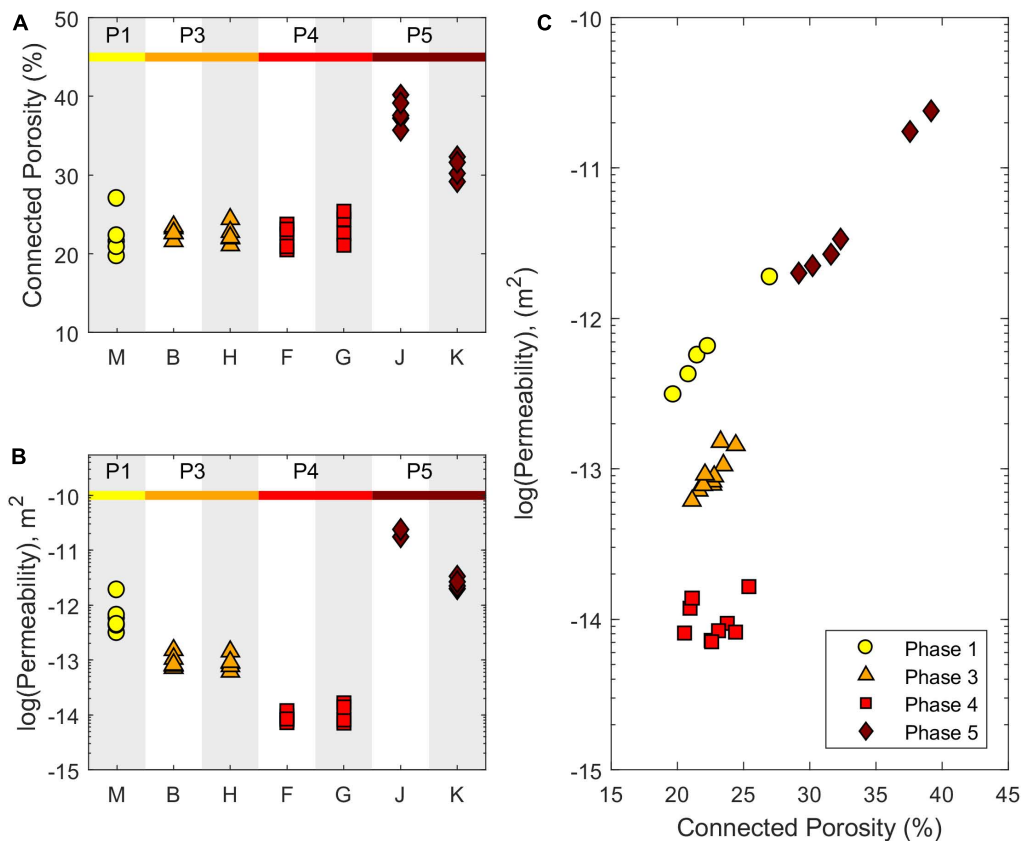
FIGURE 6 | Physical properties of 26 mm cores from eruptive Phases 1, 3, 4, and 5: (A) connected porosity evolution and (B) gas permeability evolution throughout the eruption; (C) permeability as a function of porosity for all samples. Results show that porosity is consistent between Phases 1, 3, 4, and increases in Phase 5, whereas permeability systematically decreases from Phase 1 through to Phase 4, and then increases in Phase 5. Phases 1 and 5 follow a near-continuous trend on the porosity-permeability plot, while Phases 3 and 4 plot distinctly, suggesting contrasting pore morphology and connectivity.
