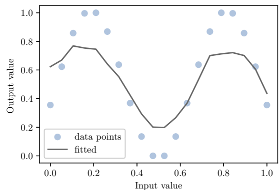
Figure 5: Original data points (sample size of 20) for the Griewank function with one-dimensional input data and the quantum surrogate function that has been obtained by running 100 optimization iterations on our ansatz (see figure 1) with six layers on the ibmq_belem QPU.
