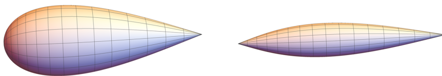
Isometric embeddings of \mathbb{CP}(3,1) and \mathbb{CP}(5,3)
