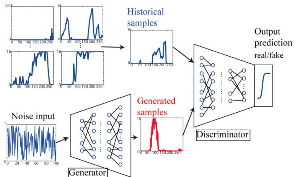
Figure 2. Architecture of GANs training procedure according to Chen et al. (2018, p. 2) .
