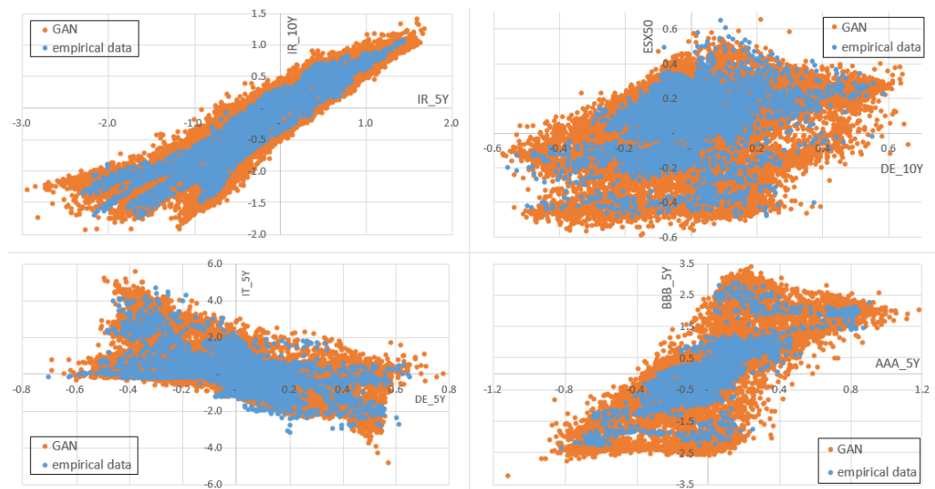
Figure 4. Scatterplots of four different risk factor pairs: empirical vs. generated data by a GAN.
