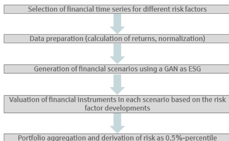
Figure 6. Workflow of a GAN-based internal model.
