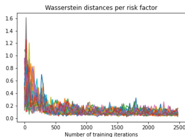
Figure 16. Development of the Wasserstein distances for all 46 risk factors during GAN training iterations.
