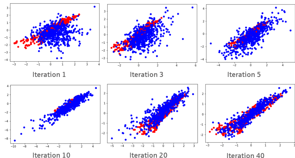
Figure 3. Scatterplots of results of a GAN for a two-dimensional data distribution at different training iterations: red = empirical data; blue = generated data.
