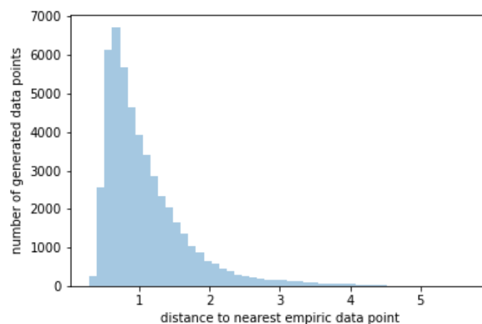
Figure 5. Histogram of minimum distances of the generated data points to the empirical data points.
