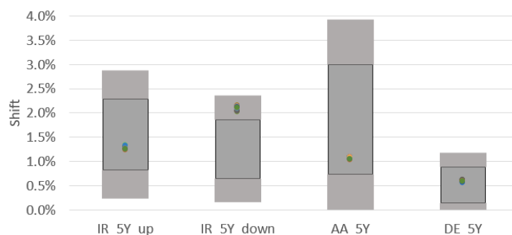
Figure 15. Comparison of the GAN risk charges in 20 different runs versus MCRCS study for four risk factors.
