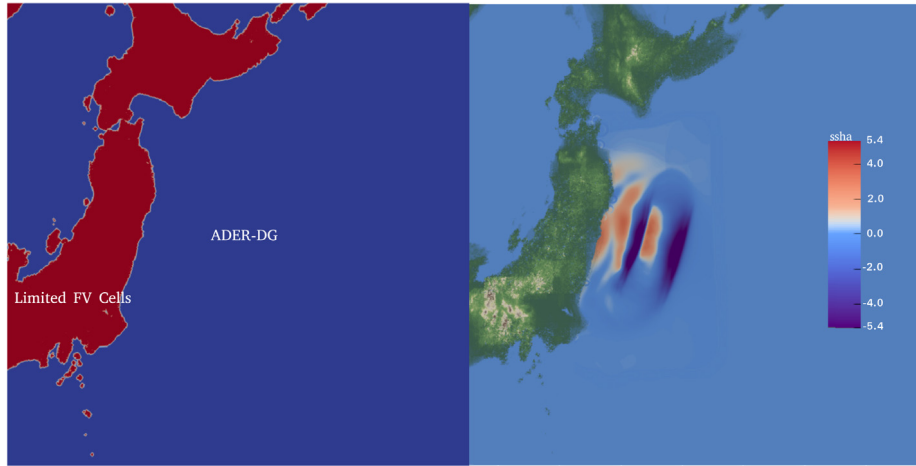
Fig. 4. Vtk output of a shallow water simulation of the Tohoku tsunami. Left: FV and DG domains. Right: the tsunami 5 min after the initial event. Source: These figures are taken from [47].
