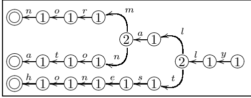
Figure 2: Lexicon trie reversely storing the entries normally , atonally and honestly . The nodes are labelled according to their SV (not normalized here). The SV peaks correspond to the boundaries of the morphemes al and ly , respectively.
