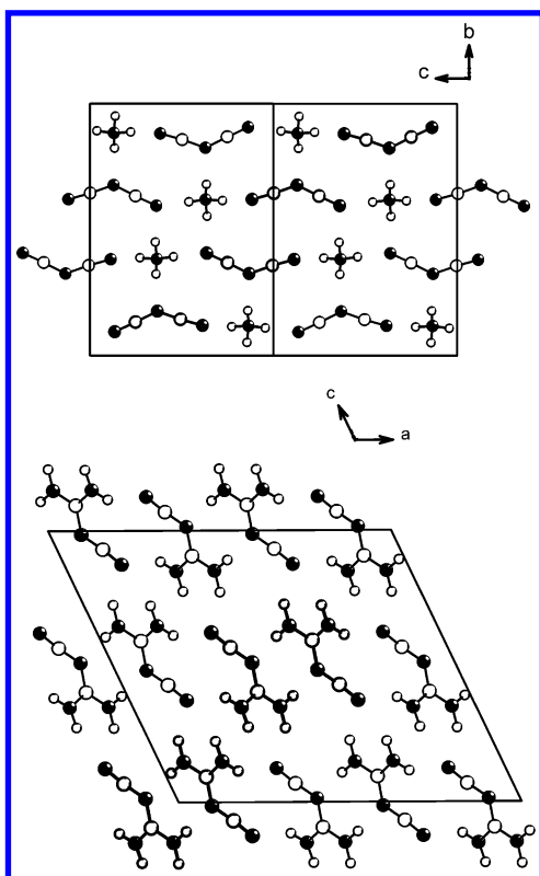
Figure 4. Top: Unit cell of ammonium dicyanamide with doubled c axis, viewed along [100]. Bottom: Unit cell of dicyandiamide, viewed along [010]. The spatial orientation of the unit cells is based on the orientation matrixes of the single crystals and therefore illustrates the relative orientation of the reactants during the transformation. According to this representation, the reorientation of the molecules takes place in the molecular planes (paper plane) of the reactants.
