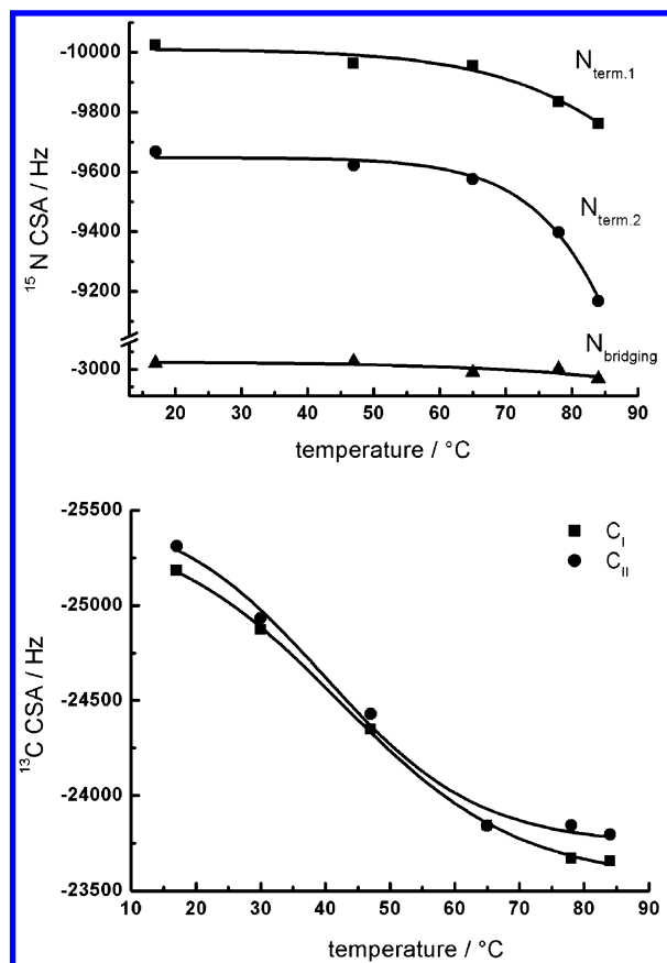
Figure 9. Temperature dependence of the chemical shift anisotropy CSA in a temperature range from room temperature to 87 °C. Top: ^{15}\text{N} , spinning rate 1.5 kHz. Bottom: ^{13}\text{C} , spinning rate 5 kHz.
