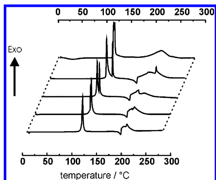
Figure 1. DSC curves showing the thermal behavior of \text{NH}_4[\text{N}(\text{CN})_2] between room temperature and 300 °C at heating rates 0.5, 1, 2, 5, and 7 °C \text{min}^{-1} . For better visualization, an x-axis offset of 8 °C for each curve was chosen.
