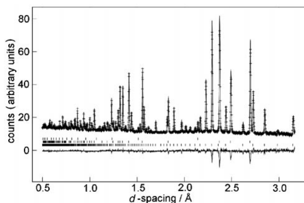
Fig. 2 Observed (crosses) and calculated (line) TOF neutron powder diffraction pattern as well as the difference profile of the Rietveld refinement. The lower row of vertical lines indicates possible peak positions of Sr 3 Pr 10 Si 18 Al 12 O 18 N 36 (upper row: vanadium of the sample container; middle row: AlN impurities).
