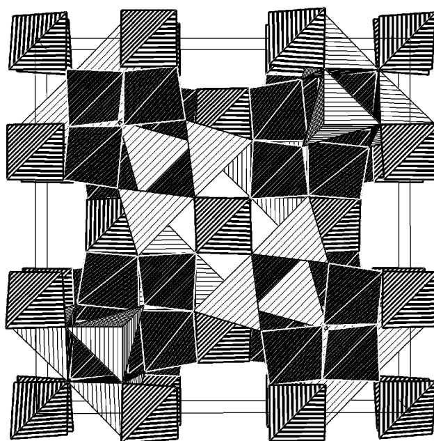
Fig. 4 {}^3_{\infty}[(\text{Si}_{18}\text{Al}_{12}\text{O}_{12}\text{N}_{12}\text{N}_{24})] network of the sialons \text{Sr}_3\text{Ln}_{10}\text{Si}_{18}\text{Al}_{12}\text{O}_{18}\text{N}_{36} (Ln = Ce, Pr, Nd) consisting of \text{SiO}_4 (black), \text{AlO}_4 (grey), and \text{SiN}_4 tetrahedra (dark hatched).
