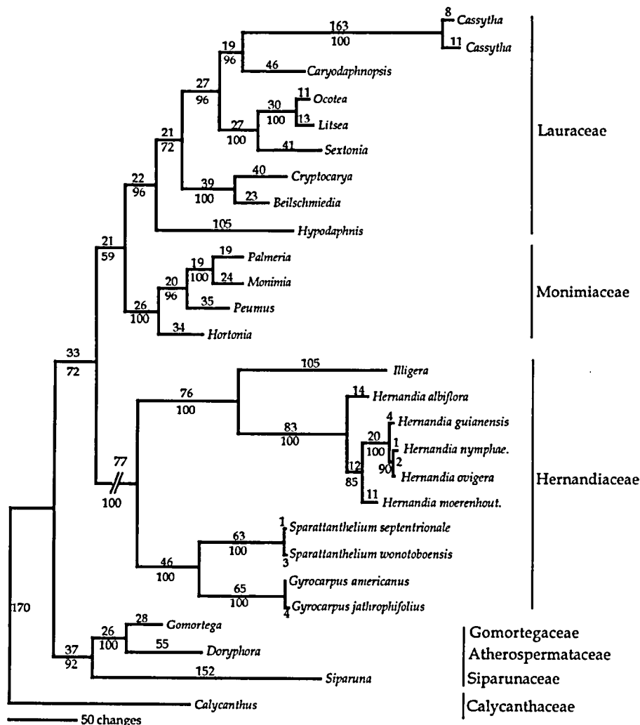
Fig. 3 The single most parsimonious tree for Hernandiaceae, Lauraceae, and Monimiaceae (length = 1969 steps, consistency index = 0.70, retention index = 0.74). Figures above branches give the number of substitutions along a branch; figures below branches are bootstrap values based on 1000 replicates. The branch leading to Hernandiaceae is shortened by one-half.
