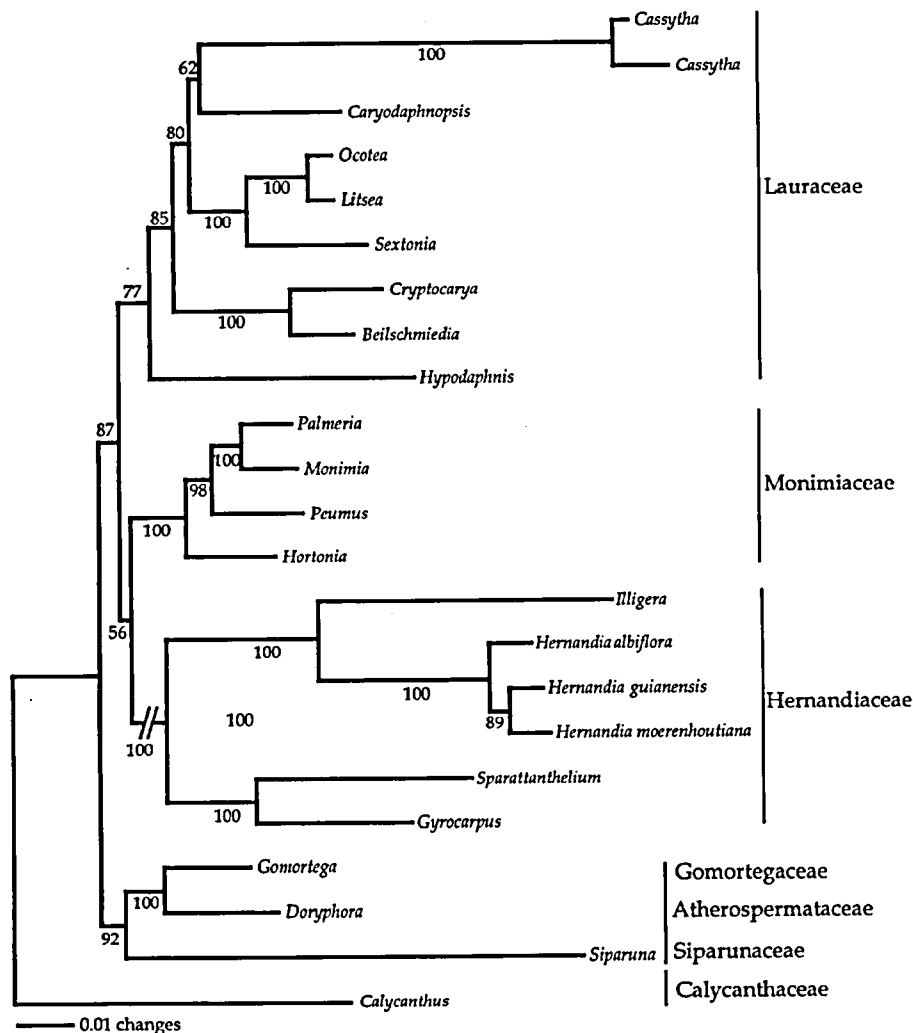
Fig. 2 Minimum evolution tree, using LogDet distances for Hernandiaceae, Lauraceae, and Monimiaceae. Bootstrap values below branches are based on 1000 replicates. The branch leading to Hernandiaceae is shortened by one-half.
