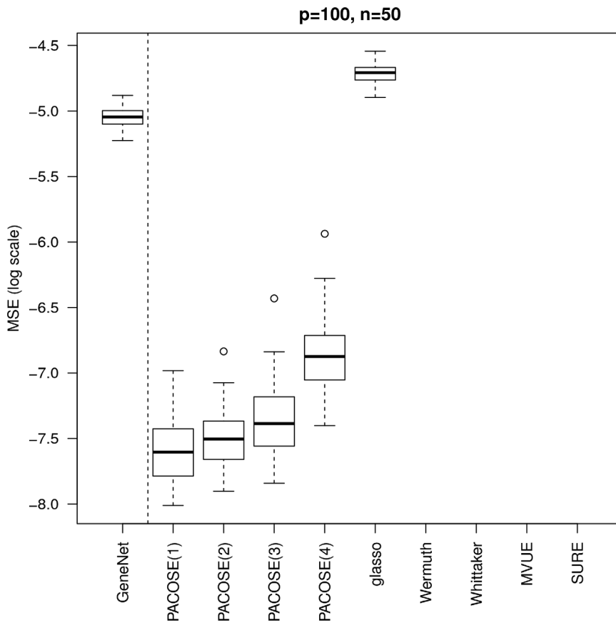
Figure 3. MSE of the partial correlation matrix estimates. p=100 and n=50 , when the graphs are not decomposable. Since the graphs are not decomposable, the estimators MVUE and SURE are not applicable. Wermuth’s algorithm does not converge, and the implementation of Whittaker’s method requires a decomposition of the graph into cliques. doi:10.1371/journal.pone.0060536.g003
