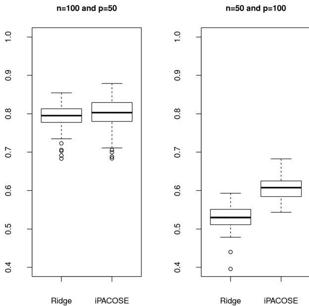
Figure 6. Measure of the stability with Fleiss' \kappa for the methods ridge.net and the Ridge version of iPACOSE. LEFT FIGURE: n=100 and p=50 . RIGHT FIGURE: n=50 and p=100 . The regularization parameter of the ridge regression is determined analytically [26] for both methods. doi:10.1371/journal.pone.0060536.g006
