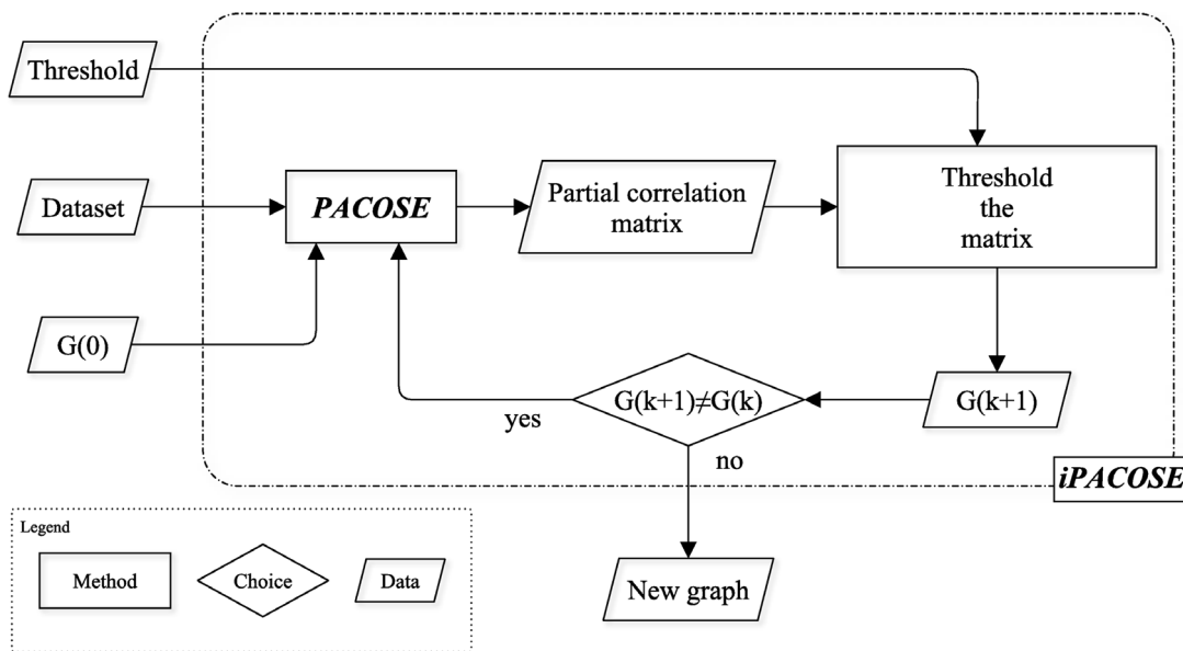
Figure 1. Flowchart representation of the iPACOSE algorithm, representing how it iteratively uses PACOSE to estimate an independence graph from a dataset. doi:10.1371/journal.pone.0060536.g001
