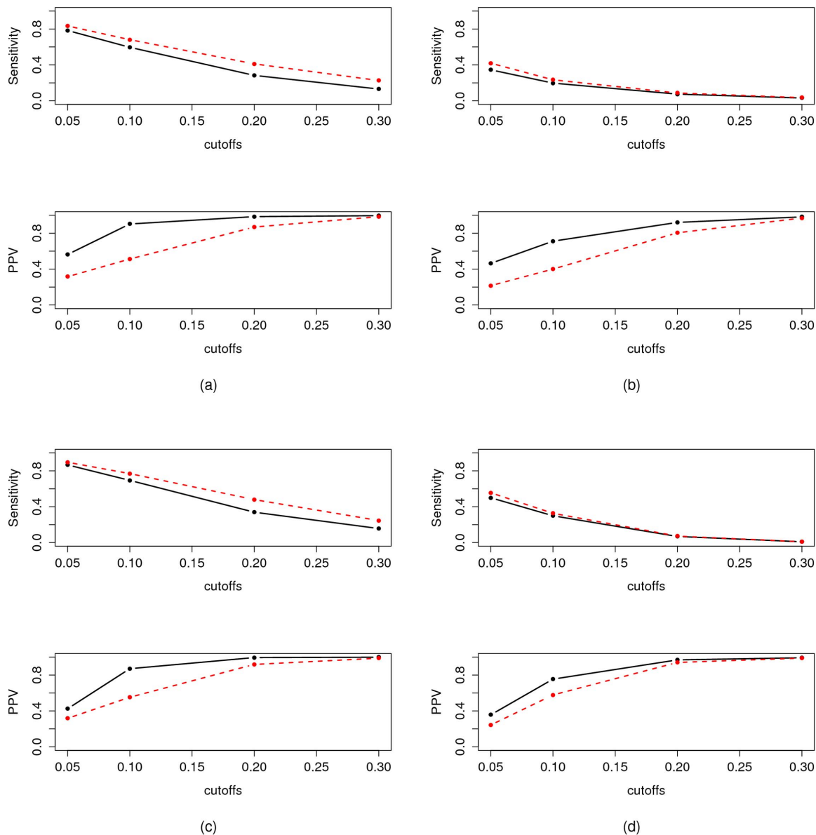
Figure 4. Performance of iPACOSE (black straight lines) when compared to its regression based GGM estimate counterpart (red dashed lines). (a) and (b): performance of the PLS version of iPACOSE. sen and ppv for p=100 and n=50 (a) and for p=50 and n=100 (b). Thresholds: 0.05, 0.1, 0.2 and 0.3. The results of iPACOSE are represented by the black line and the results of the pls.net function with the red dashed line. UPPER FIGURE : sensitivity as a function of the threshold, LOWER FIGURE : PPV as a function of the threshold. (c) and (d): performance of the Ridge version of iPACOSE. sen and ppv for p=100 and n=50 (c) and for p=50 and n=100 (d). Thresholds: 0.05, 0.1, 0.2 and 0.3. The results of iPACOSE are represented by the black line and the results of the ridge.net function with the red dashed line. UPPER FIGURE : sensitivity as a function of the threshold, LOWER FIGURE : PPV as a function of the threshold. doi:10.1371/journal.pone.0060536.g004
