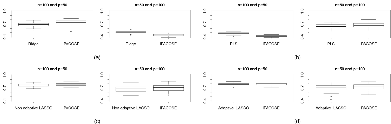
Figure 7. Measure of the stability with Fleiss' \kappa for (a) ridge.net and the Ridge version of iPACOSE, (b) pls.net and the PLS version of iPACOSE, (c) the non adaptive version of the method adalasso.net and the LASSO version of iPACOSE and (d) the adaptive version of the method adalasso.net and the adaptive LASSO version of iPACOSE. For each one of the couples of figures, the LEFT FIGURE corresponds to n=100 and p=50 and the RIGHT FIGURE to n=50 and p=100 . The regularization parameters of the Ridge, PLS, LASSO and adaptive LASSO regressions are determined analytically via a 5-fold cross-validation. doi:10.1371/journal.pone.0060536.g007
