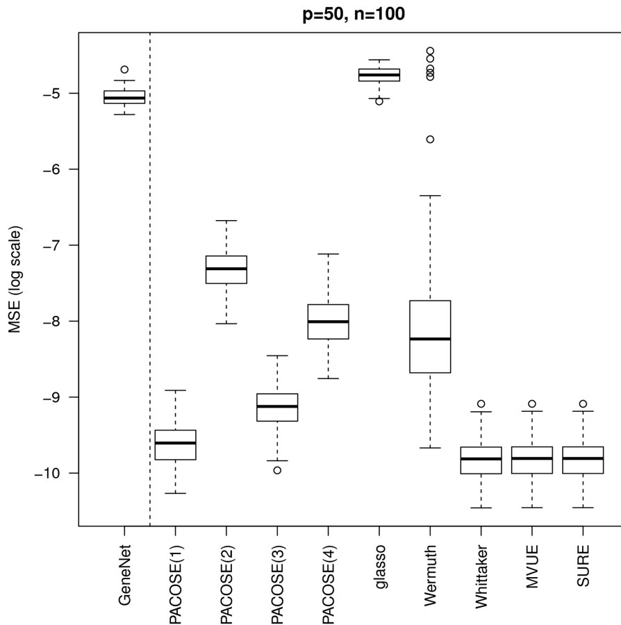
Figure 2. MSE of the partial correlation matrix estimates. p = 50 and n = 100 , when the graphs are decomposable. doi:10.1371/journal.pone.0060536.g002
