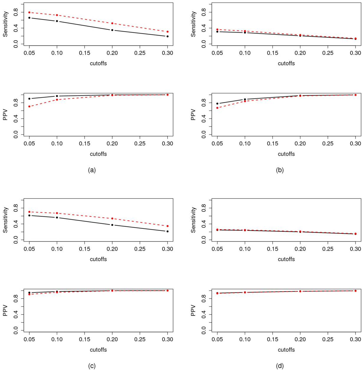
Figure 5. Performance of iPACOSE (black straight lines) when compared to its regression based GGM estimate counterpart (red dashed lines). (a) and (b): performance of the LASSO version of iPACOSE. sen and ppv for p=100 and n=50 (a) and for p=50 and n=100 (b). Thresholds: 0.05, 0.1, 0.2 and 0.3. The results of iPACOSE are represented by the black line and the results of the adalasso.net function with the red dashed line. UPPER FIGURE : sensitivity as a function of the threshold, LOWER FIGURE : PPV as a function of the threshold. (c) and (d): performance of the adaptive LASSO version of iPACOSE. sen and ppv for p=100 and n=50 (c) and for p=50 and n=100 (d). Thresholds: 0.05, 0.1, 0.2 and 0.3. The results of iPACOSE are represented by the black line and the results of the adalasso.net function with the red dashed line. UPPER FIGURE : sensitivity as a function of the threshold, LOWER FIGURE : PPV as a function of the threshold. doi:10.1371/journal.pone.0060536.g005
