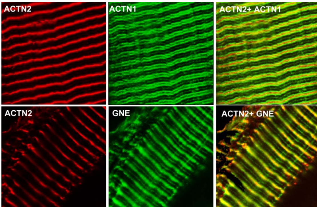
Figure 7. GNE and \alpha -actinin 1 are expressed in stretched mouse muscle. Confocal microscopy of stretched mouse spinalis muscle stained with antibodies recognizing the Z line marker \alpha -actinin-2 (ACTN2, red), \alpha -actinin-1 (ACTN1, green), and GNE (GNE, green). \alpha -Actinin-1 antibodies(3A2) and GNE antibodies show a distinct but overlapping staining pattern: GNE Abs recognize a diffuse band centered on the Z line while \alpha -actinin-1 Abs stain two distinct bands on either side of the Z line. Both Abs recognize also, as a fainter staining, the sarcomeric M line. Overlap stain between \alpha -actinin-1 and \alpha -actinin-2 Abs is minimal. doi:10.1371/journal.pone.0002477.g007
