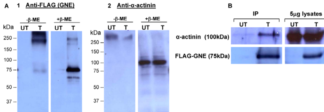
Figure 5. \alpha -Actinin is co-immunoprecipitated with FLAG-GNE in 293T-FG cells. [A] Western blot analyses with anti-FLAG antibody (A1) and anti- \alpha -actinin antibody (A2) on 5 \mu g lysate-samples of FLAG-GNE (FG)-transfected (T) and untransfected (UT) 293T cells, treated with SDS sample buffer in the presence (+) or absence (-) of \beta -ME. [B] Co-IP results. Western blot analyses with anti-FLAG antibody and anti- \alpha -actinin antibody of IP eluates and 5 \mu g lysate-samples, of FLAG-GNE (FG)-transfected (T) and untransfected (UT) 293T cells. doi:10.1371/journal.pone.0002477.g005
