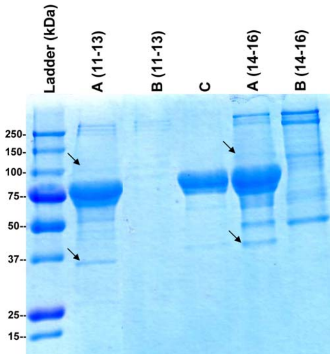
Figure 2. LDH-B and \alpha -actinin 1 precipitate with GNE by in vitro binding assay. Gelcode reagent staining of in vitro binding assay eluates resolved by SDS-PAGE. Numbers (11–13, 14–16) correspond to anion-exchange pooled fractions. A, proteins bound to GNE-bound nickel beads; B, proteins bound to GNE non-bound nickel beads; C, control proteins bound to GNE-bound nickel beads. Black arrows point to either \alpha -actinin 1 (~100 kDa) or LDH-B (~37 kDa). Both proteins were identified by MS (Table 1). doi:10.1371/journal.pone.0002477.g002
