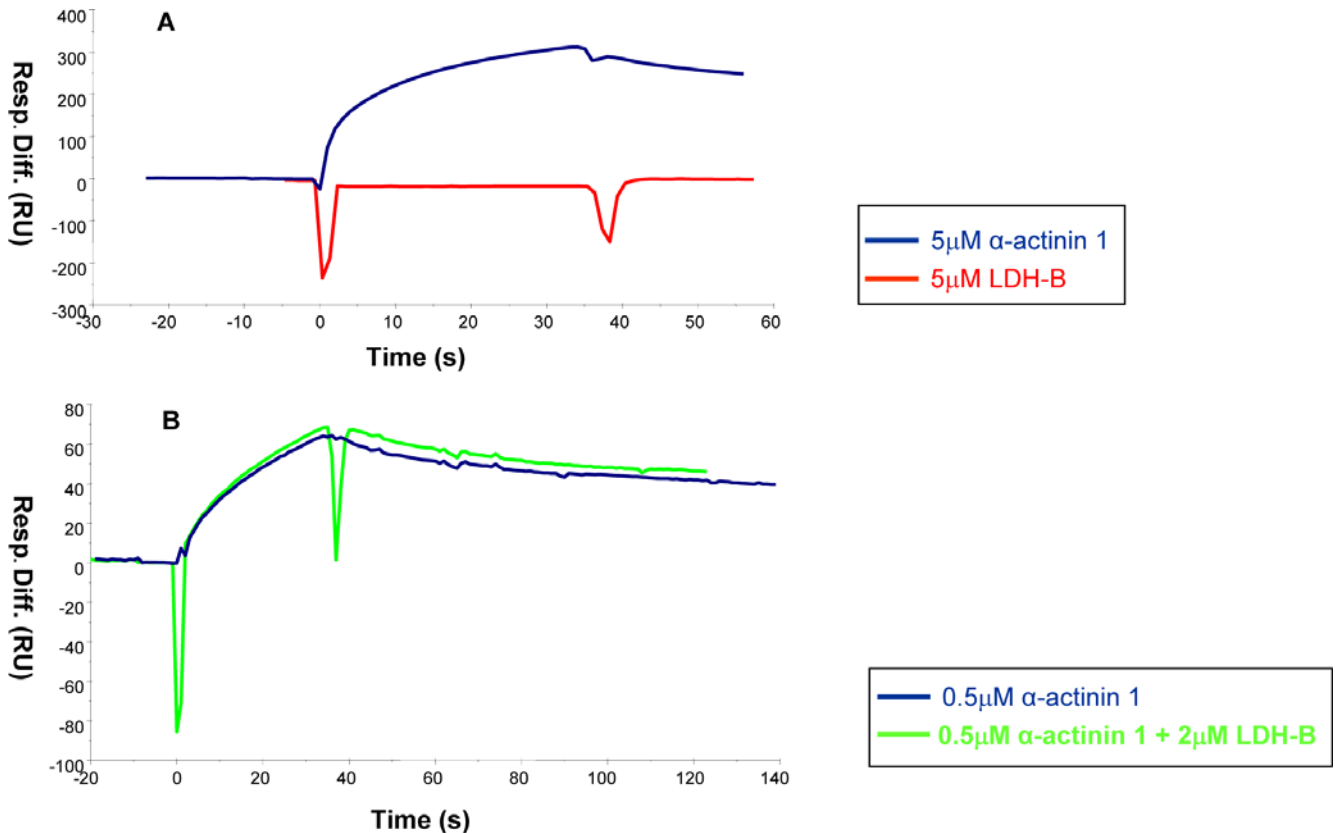
Figure 4. LDH-B does not show BIAcore binding signal with GNE. [A] Sensorgram of the interaction of GNE with 5 \mu M LDH-B, compared to 5 \mu M \alpha -actinin 1. [B] Sensorgram showing the effect of 2 \mu M LDH-B on the interaction of GNE with 0.5 \mu M \alpha -actinin 1 [Resp. Diff., response difference; RU, response units]. doi:10.1371/journal.pone.0002477.g004
