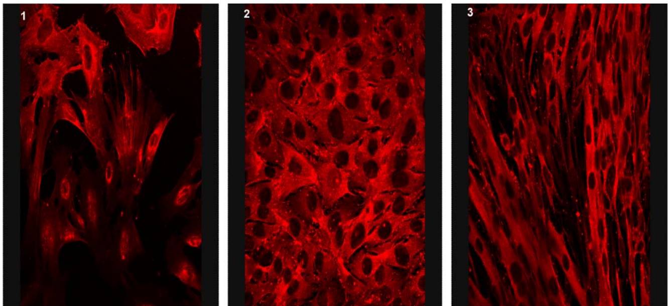
Figure 6. \alpha -Actinin 1 is expressed in skeletal muscle. Light microscopy of mouse muscle culture (C2C12) at differentiation day (DD) 0 (1), DD 1 (2) and DD 3 (3) stained with antibody to \alpha -actinin-1 (3A2). doi:10.1371/journal.pone.0002477.g006
