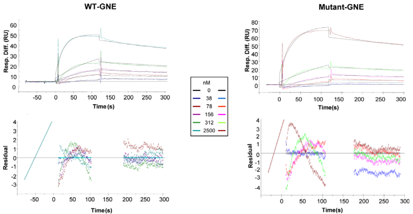
Figure 3. WT and mutant GNE proteins interact with \alpha -actinin 1. Sensorgrams showing the interactions of GNE (WT and mutant) proteins with different \alpha -actinin 1 concentrations and the residual curves, showing the fitness between the model and the experimental results [Resp. Diff., response difference; RU, response units]. doi:10.1371/journal.pone.0002477.g003
