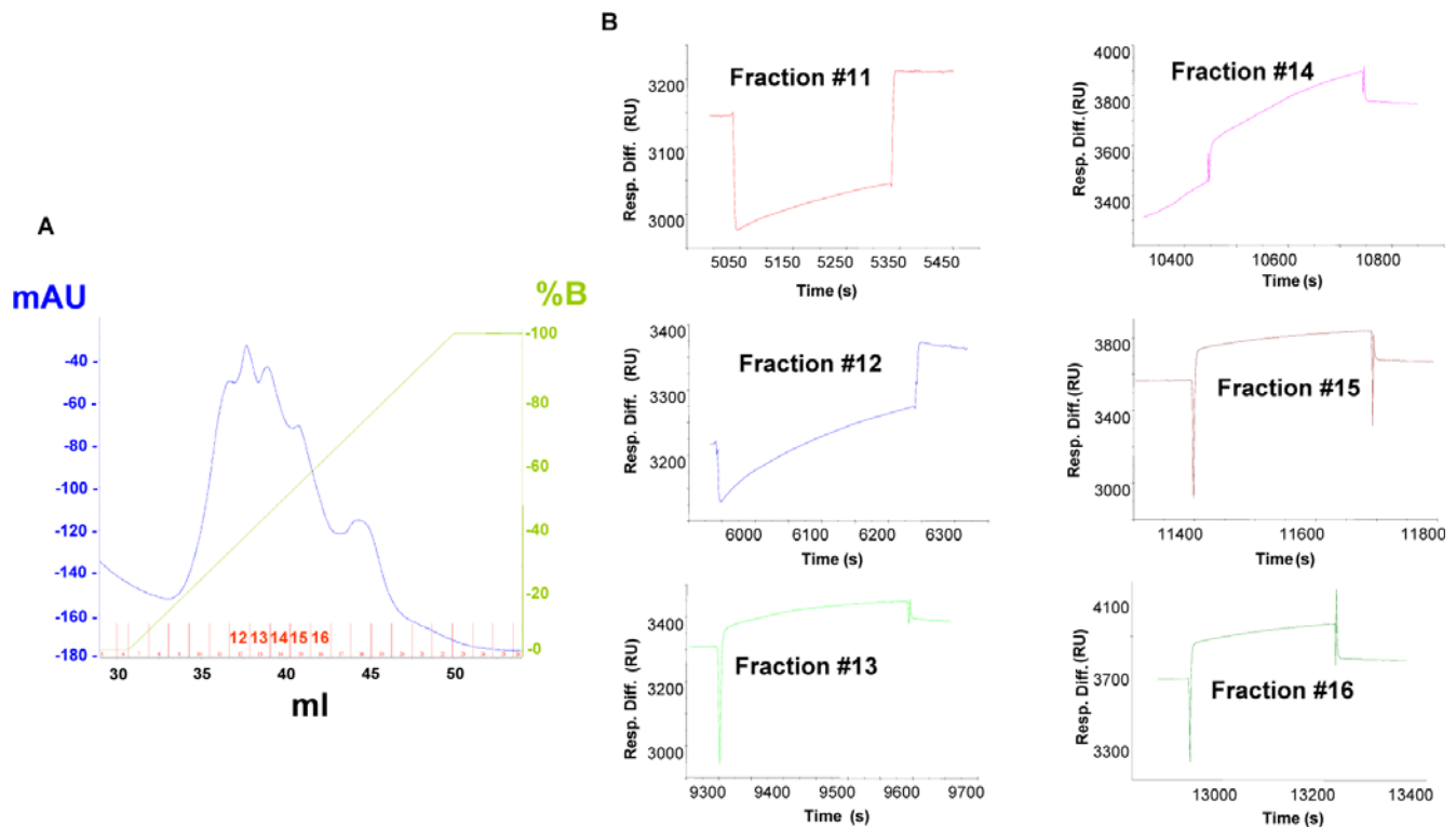
Figure 1. WT-GNE interacts with proteins within anion-exchanged fractions of muscle cell lysate. [A] Anion exchange chromatography (0–1 M NaCl) of cell lysate (15 mg total protein content) extracted from human skeletal muscle primary culture cells. The numbers of the positive fractions appear in red on the X axis. [B] BIAcore sensorgrams of the interaction of WT-GNE with anion exchange fractions #11–16 [Resp. Diff., response difference; RU, response units; B, buffer B (see Materials and methods)]. doi:10.1371/journal.pone.0002477.g001
