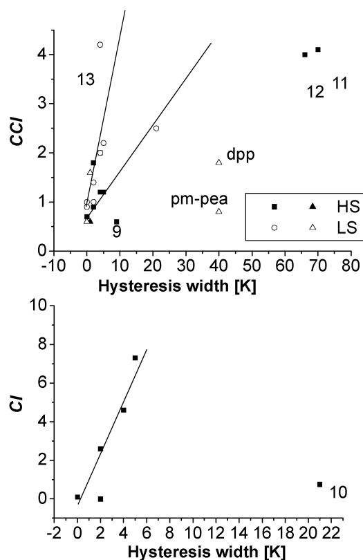
Fig. 7 Plots of the crystal contact index (CCI) (top) and the crystal index (CI) (bottom) against the hysteresis width. Values are taken from Table 4 (circles and squares) and from the text (triangles, literature examples).
