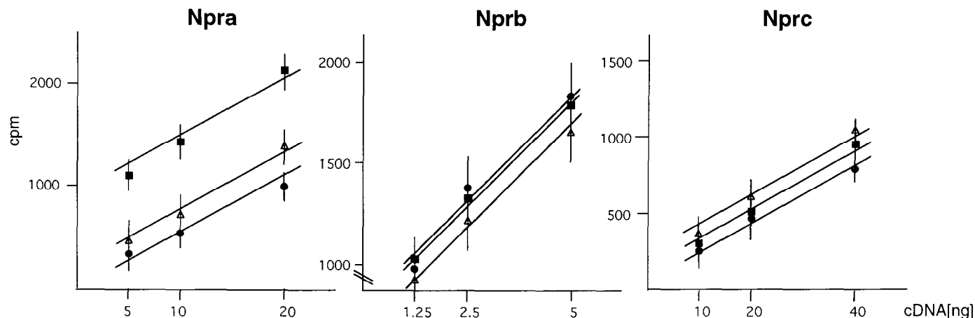
FIG. 5. Graphic line of incorporated radioactivity (cpm) of PCR amplification products blotted against the amount of initial cDNA. Levels of Npra, Nprb, and Nprc transcripts in native (●), cultured (△), and Con A (■) stimulated thymocytes are indicated by the amount of incorporated radioactivity (cpm) as described in Materials and Methods . Each value represents the mean of three independent experiments ( \pm SD) run in triplicates.
