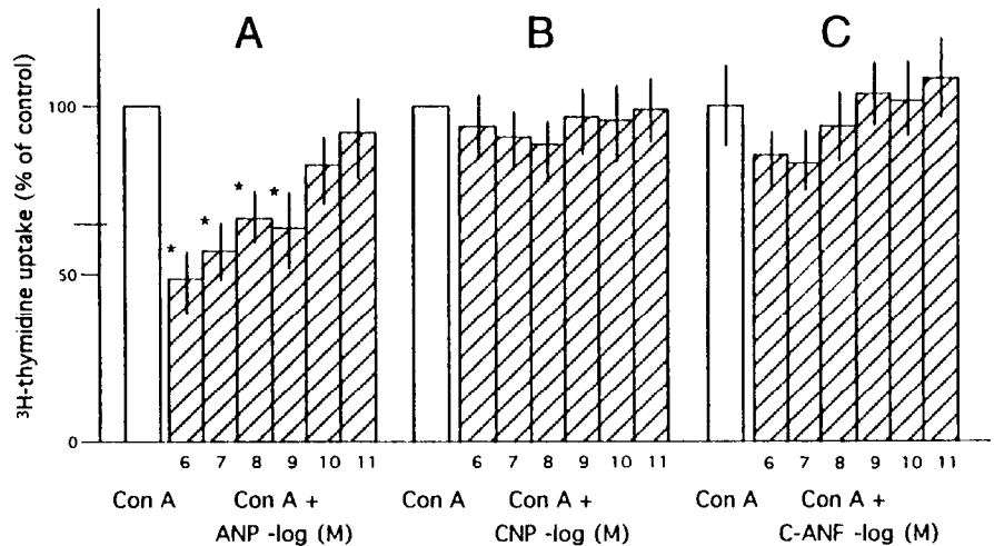
FIG. 7. Effects of NP on Con A-stimulated incorporation of [ ^3 H]thymidine in thymocytes. Cells ( 2 \times 10^5 /well) were treated with Con A ( 1 \mu\text{g}/\text{ml} , 48 h) with or without decreasing concentrations ( 10^{-6} M– 10^{-11} M) of ANP (panel A), CNP (panel B), and C-ANF (panel C). Thymocytes were then pulsed with [ ^3 H]thymidine ( 1 \mu\text{Ci}/\text{well} ) for another 15 h. Values are normalized to levels found in Con A-stimulated cells (100%) and are given as means \pm SD, n = 6 –12. *, P < 0.05 , t test. Each experiment was performed at least four times.
