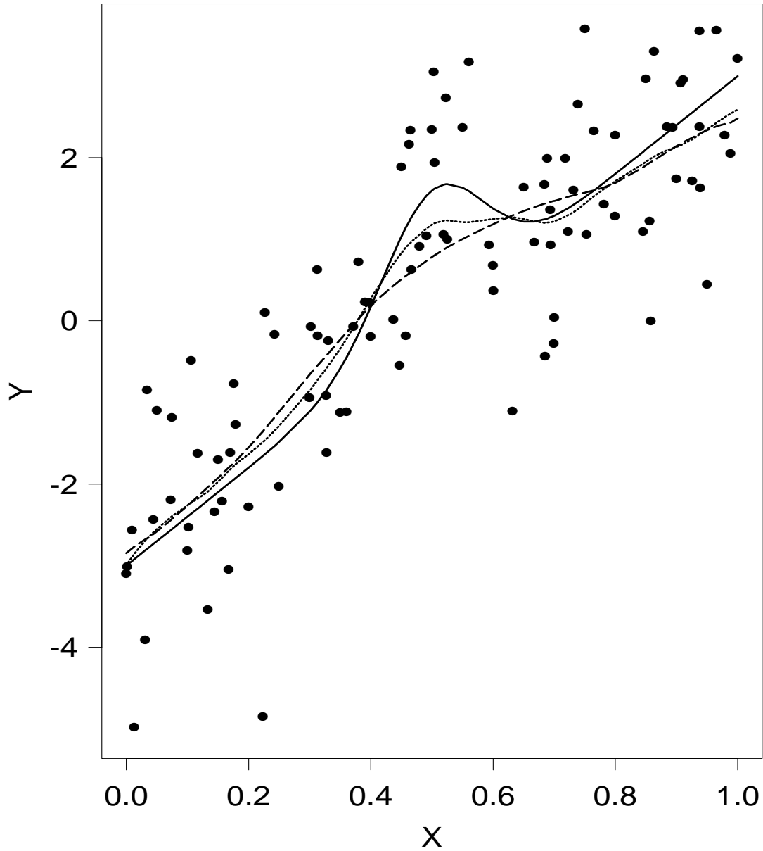
Figure 1: True value of E(Y|X) = m_2(X) = (2\pi)^{-1/2}4(X - 0.5) + 4\exp[-2\{4(X - 0.5)\}^2] , denoted by the solid line, along with the estimates \widehat{m}_{2h}(X) and \widehat{m}_{2g}(X) , in dotted and dashed lines respectively.
