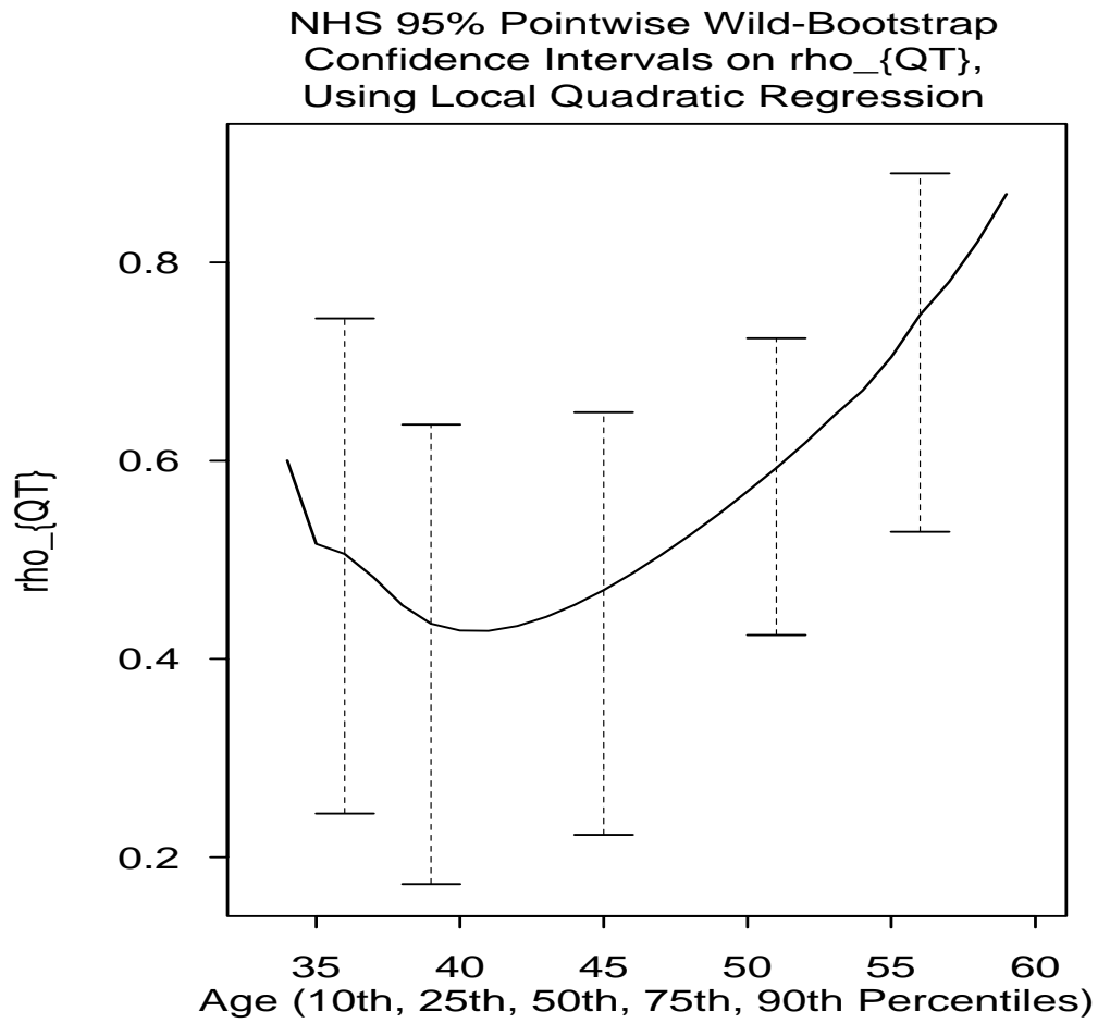
Figure 3: Nurses' Health Study percent of calories from fat, estimating \rho_{QT} using local quadratic regression, along with 95% wild-bootstrap pointwise confidence intervals on the 10th, 25th, 50th, 75th, and 90th percentiles of age.
