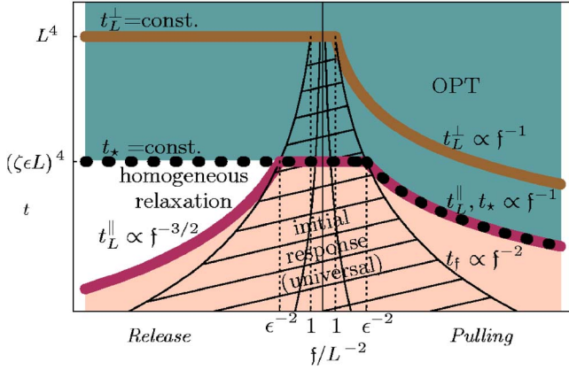
FIG. 6. (Color online) Characteristic times (logarithmic scale) for pulling and release against the applied external force f (linear scale). The time t_* (stars) separates regions where ordinary perturbation theory (OPT) applies (dark shaded) from regions (light shaded) of linear (hatched) and nonlinear tension propagation and from homogeneous tension relaxation (white). Whereas longitudinal friction is negligible for t > t_* , it limits the dynamics for t < t_* . The innermost funnel-shaped region indicates the regime where the tension fluctuations are important [defined by f < \delta f with \delta f given by Eq. (107)].
