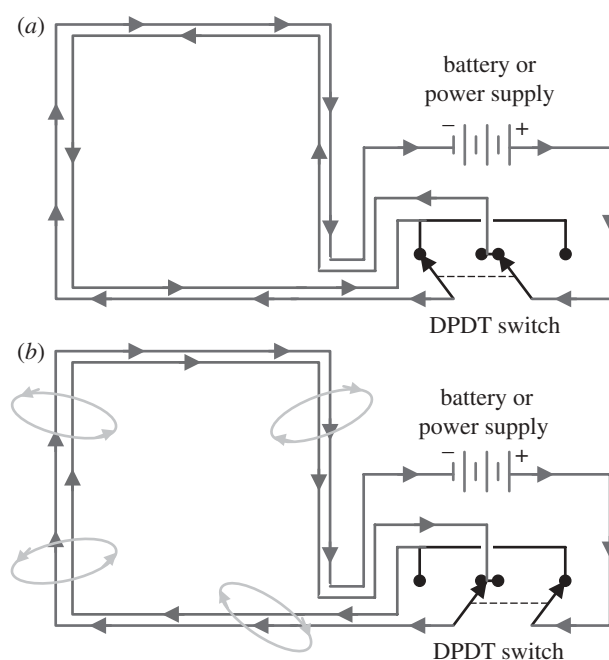
Figure 1. A simple circuit for introducing blind conditions in experiments using static or low-frequency magnetic fields, adapted from Kirschvink (1992 b ). When building the coil systems, wrap them carefully with two identical strands of wire, placed adjacent to each other and held firmly in place with high-conductivity thermal epoxy (to minimize vibration). These 'double-wrapped' coils can then be configured with a silent DPDT switch that will allow the current to flow in series through the two coils, but permits the direction of flow to be reversed in one of them. (a) Circuit with the DPDT switch set so that the current in the two coils is in opposition, yielding no external magnetic field (sham mode). (b) Same circuit with the switch set to produce parallel current flow, yielding the external magnetic field (active mode). We recommend using quasi-random Gellermann (1933) orders to set the active/sham states by a person external to the experiment. If that is impractical, a second DPDT switch can be inserted in the circuit, and two separate investigators can each control one of the switches with separate random orders to ensure fully blinded experimental conditions. Recommendations for multiple-coil designs to produce uniform magnetic stimuli within an experimental chamber are also given by Kirschvink (1992 b ).
