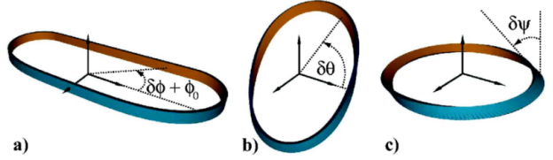
Fig. 1. Illustration of the Euler angles and their coupling induced by the ring geometry: A sinusoidal variation of each Euler angle at a time results in more than one free energy term, if coupling is present: (a) \delta\phi = \sin(s/R_c) , in-plane bending only, \bar{F} = a_1 , (b) \delta\theta = \sin(s/R_c) , transversal bending yields in-plane bending and twisting, \bar{F} = -a_1 + a_2 + a_3 , (c) \delta\psi = \sin(s/R_c) , twisting yields both in-plane and transversal bending, \bar{F} = -a_1 + a_2 + a_3 ; F in units of \pi k_B T / 2R_c .
