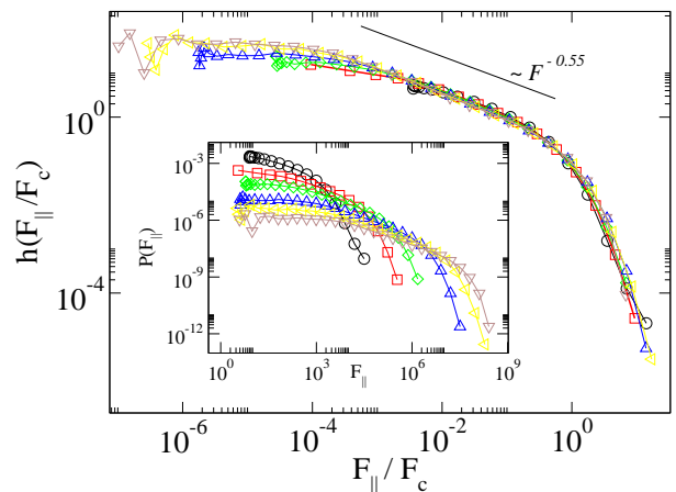
Fig. 3. Probability distribution P(F_{\parallel}) (inset) and scaling function h in the non-affine bending regime with aspect ratio r/l_f = 5 \cdot 10^{-6} for various densities \rho l_f = 20 \dots 100 . The force scale used to obtain the data collapse is F_c = \kappa \rho_c^2 (\delta \rho / \rho_c)^5 .
