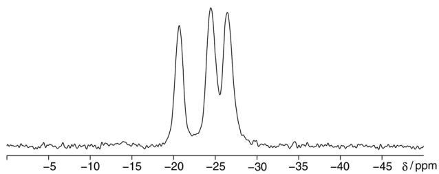
Fig. 3 Isotropic signals in a ^{31}\text{P} MAS NMR spectrum of (\text{TMA})_2\text{HP}_3\text{O}_9 obtained at a sample spinning frequency of 6 kHz. The spectrum shows three signals corresponding to three different crystallographic orbits of phosphorus atoms.
