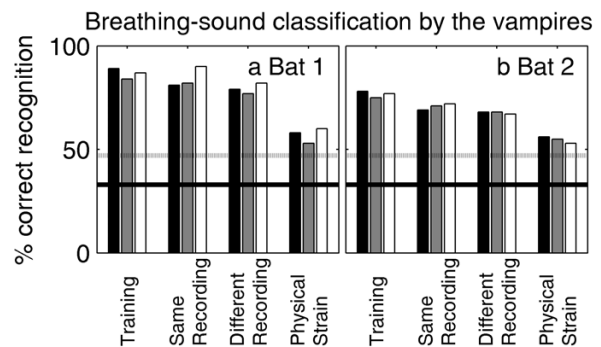
Figure 3 Spontaneous classification of unknown breathing sounds by D. rotundus . The two panels show results from two individuals. The correct recognition of a breathing sound recorded from one of three human subjects is shown as a function of the condition of breathing-sound recording. The different bar colors represent the three different subjects. The bold horizontal line at 33 % correct indicates chance level, the gray line at 47 % correct indicates significant deviation from chance with p < 0.05 . The data show that both animals recognized the breathing sounds correctly under all experimental conditions. Only under the most difficult condition, where the sounds were recorded under physical strain (unlike the training sounds), the bats' performance dropped markedly but still remained significant.
