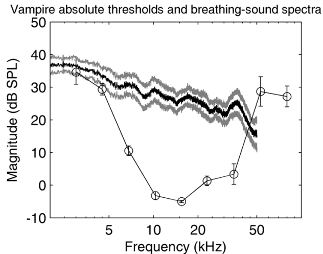
Figure 4 Vampire hearing and breathing-sound spectra. Absolute auditory thresholds averaged across three individuals of D. rotundus are shown as symbols and the fine line; error bars represent standard errors of the mean. Averaged breathing-sound magnitude spectra are shown by the strong black line; the strong grey lines again represent standard errors. This comparisons show that in D. rotundus , auditory sensitivity is well suited to detecting and analyzing breathing sounds.
