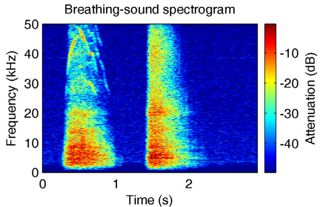
Figure 2 Spectrogram of a recorded breathing sound. The spectrogram shows the spectro-temporal features of an air intake (left) and output (right) in a single breathing-sound cycle. Frequency-modulated, ultrasonic tonal components can be observed during air intake. These components result from turbulences in the nasal cavity during depression. Note the good signal-to-noise ratio, which was realizable with the recording equipment described in the methods.
