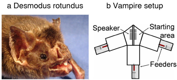
Figure 1 Animal portrait (a) and experimental setup (b) for the behavioral experiments on breathing-sound classification and absolute thresholds in the common vampire bat, Desmodus rotundus . For the breathing-sound classification, animals were trained to associate each of three breathing sounds, presented from a speaker above the starting area, with one of the three feeders. For the absolute-threshold measurements, stimuli were presented from one of three speakers mounted above the feeders.
