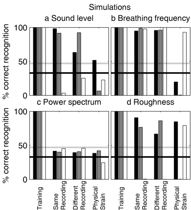
Figure 6 Numerical simulation of the breathing-sound recognition. The simulations are based on four different breathing-sound parameters, namely (a) the sound level, (b) the breathing frequency, (c) the power spectrum of the breathing sounds and (d) the breathing-sound roughness. None of the simulations matches the behavioral performance of the vampire bats (Fig. 3). The breathing-sound simulation, however, matches the performance of the naïve human listeners (Fig. 5a), confirming the listeners' reports that they had tried to rely on breathing-frequency information.
