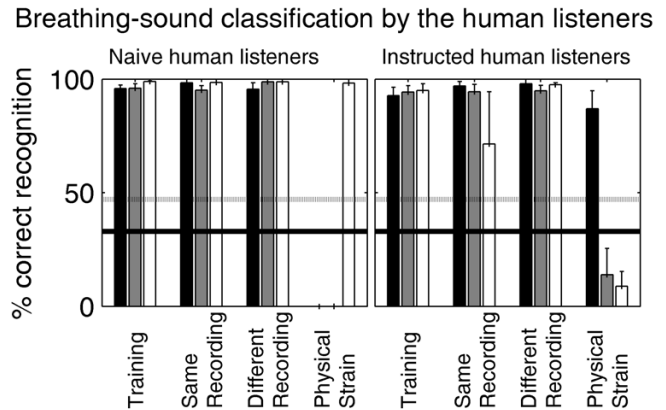
Figure 5 Breathing-sound classification by human listeners with exactly the same stimuli and experimental procedure as used in the vampire experiment. Results are shown in the same format as in Fig. 3. Error bars represent across-listeners standard errors. While the human listeners were well capable of recognizing breathing sounds recorded in the same session or in a different session in the same physical state, the naïve human listeners failed to recognize the breathing sounds recorded under physical strain (a). Even after the listeners were instructed to ignore breathing-frequency information (b), overall performance did not improve for this most difficult experimental condition.
