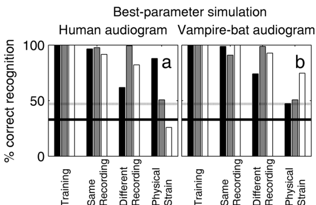
Figure 7 Simulation of the breathing-sound recognition with dynamically changing analysis parameters. Predicted breathing-sound classification when the model was free to choose the breathing-sound parameter (sound level, power spectrum or roughness) that provides the strongest predictions (strongest deviations from chance performance) for a given comparison of a test sound with each of the three training sounds. All sounds were filtered to match either the human audiogram (a) or the vampire-bat audiogram (b). While the simulation based on the human audiogram does not yield improved predictions of the classification of the test sounds recorded under physical strain, this simulation approach when combined with the sounds as they are weighted by the vampire-bat audiogram results in qualitatively correct classifications even of the test sounds recorded under physical strain.
