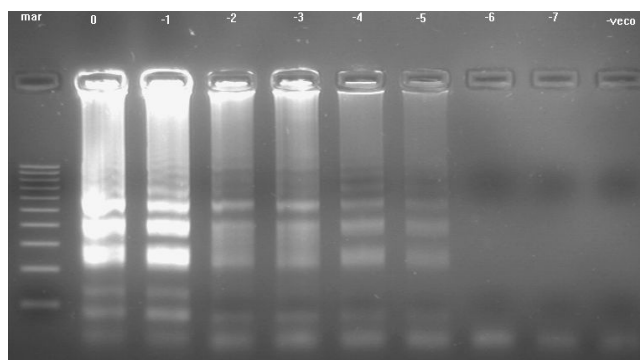
Figure 8 Agarose gel demonstrating the sensitivity of the LAMP assay using 10-fold serial dilutions of KHV DNA extracted from a clinical sample. The amplification shows a ladder-like pattern, and detected KHV DNA in a clinical sample at a dilution of 10 -5 . Lanes: 0 = undiluted KHV DNA; -1 = dilution of 10 -1 ; -2 = 10 -2 and so on; mar = 100 bp DNA molecular weight standard. -veco = negative control.
