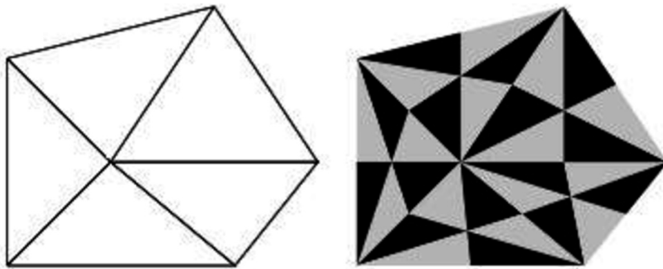
Figure 2. Barycentric subdivision.
