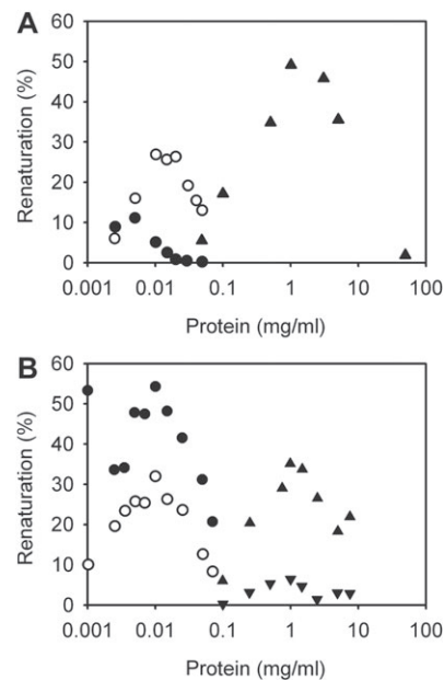
Figure 1 Matrix-assisted refolding of \alpha -glucosidase. (A) Yield of renaturation of wildtype \alpha -glucosidase and \alpha -glucosidase fused to a hexaarginine tag at its C-terminus. Renaturation was performed in 10 mM phosphate pH 7.6, 30 mM NaCl, 8% (w/v) ethylene glycol, 10°C either in solution (open circles wildtype \alpha -glucosidase; closed circles \alpha -glucosidase-Arg 6 ) or with the protein immobilized on heparin-sepharose (closed triangles). Data taken from Stempfer et al., 1996b. (B) Yield of renaturation of wildtype \alpha -glucosidase and \alpha -glucosidase fused to a decaglutamate tag at its C-terminus. Renaturation was performed in 10 mM phosphate pH 7.6, 1 mM EDTA, 10°C either in solution (open circles wildtype \alpha -glucosidase; closed circles \alpha -glucosidase-Glu 10 ) or with the protein immobilized on Fractoprep DEAE (closed triangles up) or Q-sepharose (closed triangles down). Richter and Lilie, unpublished results.
