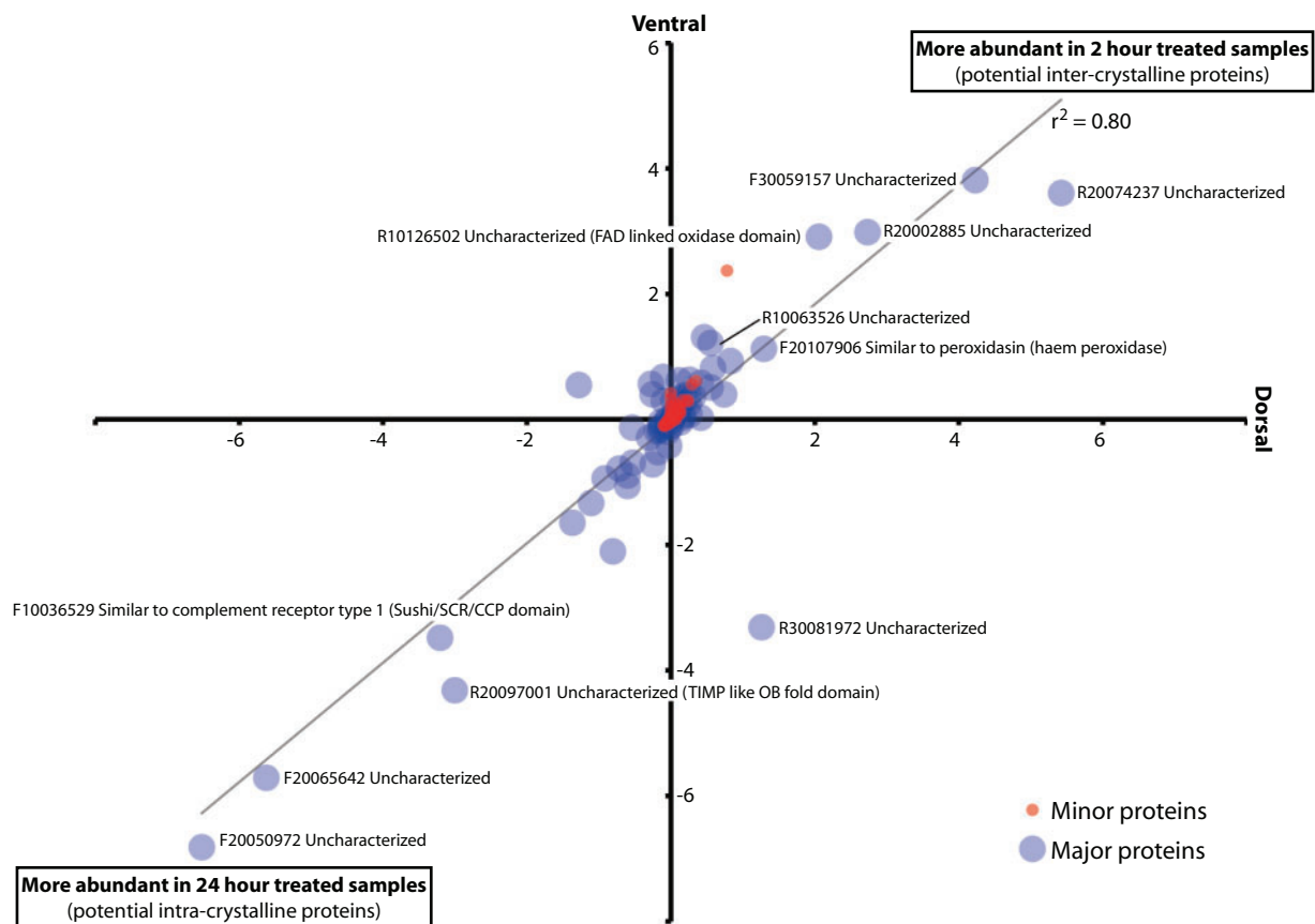
FIG. 5. —Effect of 2- versus 24-h sodium hypochlorite treatment on the abundance of proteins in dorsal and ventral shell valves. The relative abundances of 333 minor proteins (red circles) and 66 major proteins (blue circles) identified in M. venosa shells were compared following 2- versus 24-h treatment with sodium hypochlorite. iBAQ values for each peptide recorded after 24 h of treatment were subtracted from those recorded after 2 h of treatment. Negative values therefore indicate a higher peptide abundance in 24 h treated samples.
