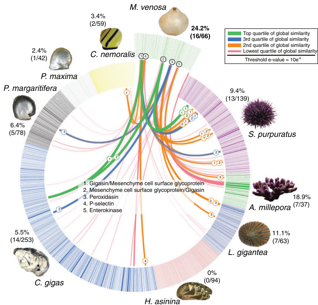
FIG. 3. —Sequence-based comparisons of M. venosa 's shell-forming proteome against other metazoan data sets. BLASTp based similarity comparison of the 66 most abundant M. venosa shell proteins against 765 shell-forming proteomes derived from eight other biocalcifying metazoans. All 66 major M. venosa shell proteins were searched against a concatenated database of shell-forming proteins derived from P. maxima and P. margaritifera (Marie et al. 2012); H. asinina ; (Marie et al. 2010); L. gigantea ; (Marie et al. 2013); C. gigas (Zhang et al. 2012), S. purpuratus (Mann et al. 2008), and A. millepora (Ramos-Silva et al. 2014) using BLASTp and an e-value cut-off of 10 \times 10^{-6} . Individual lines spanning the ideogram connect proteins that share significant similarity (e values < 10 \times 10^{-6} ). Transparent red lines connect proteins with the lowest quartile of similarity (with a threshold of 10 \times 10^{-6} ) and green lines with the highest quartile of similarity. The percentage of each shell proteome that shared similarity with the M. venosa proteome is provided.
