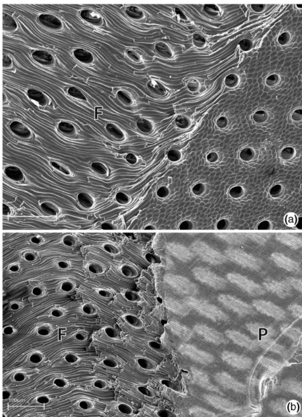
Fig. 6. —SEM images of punctae in the shell of M. venosa . (a) Punctae in a broken valve of M. venosa (view from inside of shell) with fibrous structure (F) of secondary shell layer clearly visible. (b) Punctae in a broken shell of M. venosa (view from outside of shell) at the interface of the primary (P, right side of image) and fibrous secondary layers (F, left side of image).
