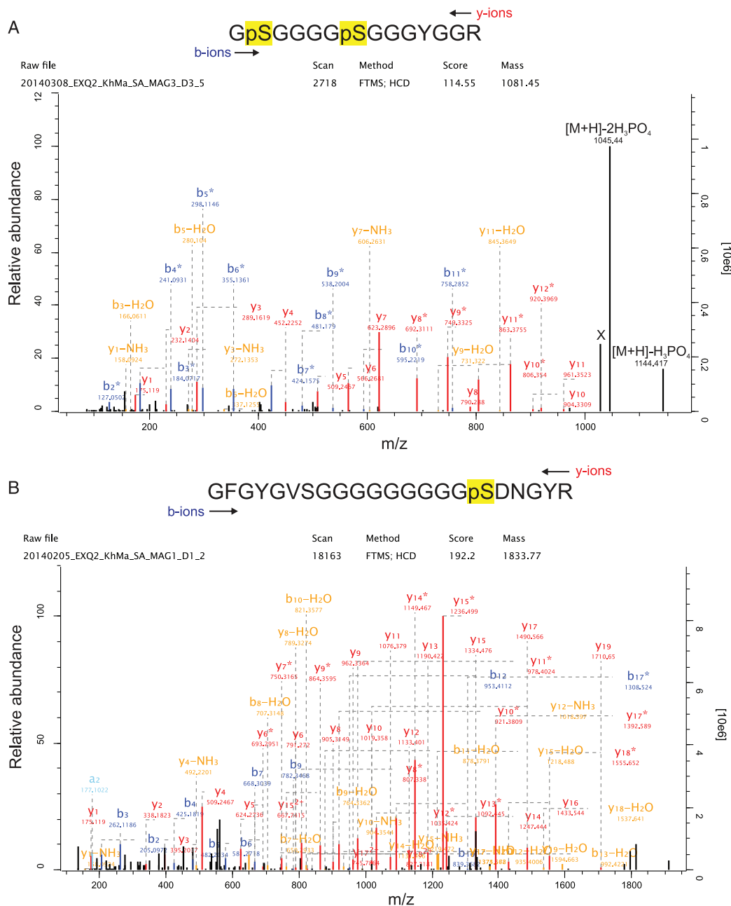
Fig. 4. —Spectrum of the major phospho-peptides of R10063526 and F30059157. (A) The doubly phosphorylated R10063526 peptide containing phosphorylated S 272 and S 277 of this entry was identified with a posterior error probability (PEP) of 0.0002 and a mass error of 0.7 ppm. The MaxQuant localization probability was 1 for both sites. Expert System advanced annotations (Neuhauser et al. 2012) were omitted to reduce complexity, except for the last two peaks ( m/z 1,144.41 and 1,045.44). Peak X was not annotated by the expert system but most probably represents [M+H]-2H 3 PO 4 -H 2 O. Y-ions are shown in red, b-ions are shown in blue, b- or y-ions with a loss of water or ammonia are in orange. Asterisks indicate loss of H 3 PO 4 . (B) The singly phosphorylated F30059157 peptide (S 174 ) was identified with a mass error of 0.7 ppm, a PEP of 3.4e-67, and a phosphosite localization probability of 1. Y-ions are shown in red, b-ions are shown in blue, b- or y-ions with a loss of water or ammonia are in orange. Asterisks indicate loss of H 3 PO 4 . Expert System advanced annotations (Neuhauser et al. 2012) are omitted for clarity of presentation.
