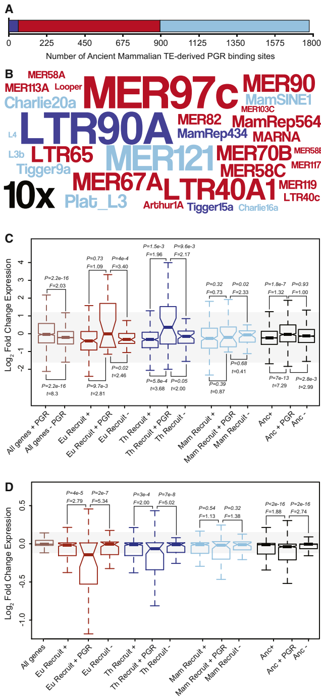
Figure 7. Ancient Mammalian TEs Globally Remodeled PGR Binding Site Architecture across the Genome (A) The number of PGR ChIP-seq peaks that contain Mammalian-specific (light blue), Therman-specific (blue), and Eutherian-specific (red) TEs in primary cultures of hESCs treated with 10 nM 17 \beta -estradiol, 100 nM medroxyprogesterone acetate, and 1 mM 8-bromo-cAMP. (B) Word cloud of ancient mammalian TEs enriched within PGR ChIP-seq peaks. Colors follow (A). Inset scale (10 \times ) shows 10-fold enrichment. Only elements with \geq 2 -fold enrichment are shown. (C) Genes associated with ancient mammalian TE-derived PGR binding sites (+ PGR) are more strongly differentially regulated in hESCs upon decidua-
