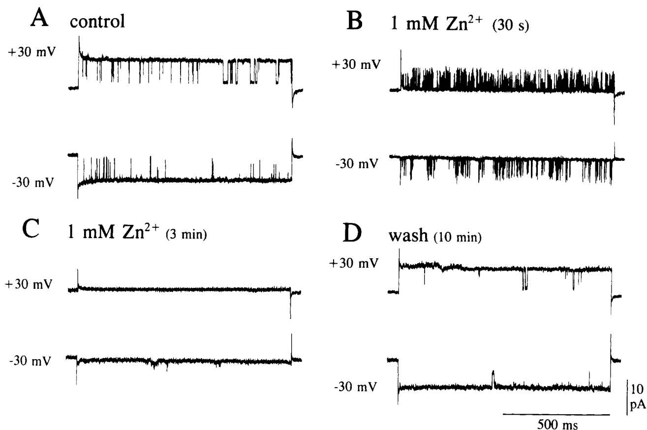
Fig. 6. Reversible block of the anion channel by \text{Zn}^{2+} . The voltage was held at 0 mV and then stepped to the pipette potentials indicated. A: Control in symmetrical solutions with 125 mM \text{K}^+ methylsulphate. B: 1 mM \text{Zn}^{2+} applied for 30 s caused rapid current fluctuations between open and closed states. After about 3 min a complete block of the anion channel was observed (C). This effect was reversible after 10 min in the control solution (D).
