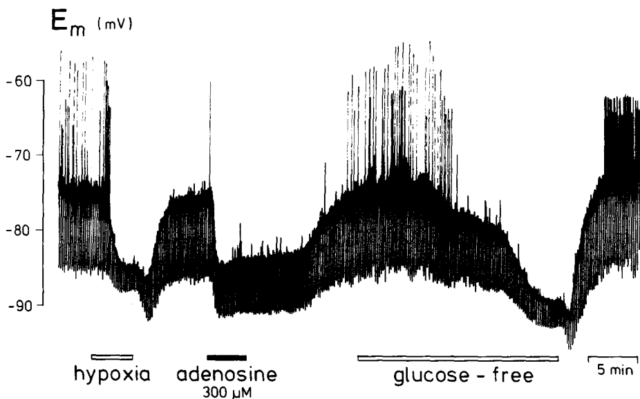
Fig. 1. Effects of energy deprivation and adenosine (300 \mu M) on membrane potential ( E_m ) and input resistance of a CA3 neurone in a rat hippocampal slice. Intracellular recording in current-clamp mode was performed with KCl-filled microelectrodes (3 M). For the determination of input resistance, hyperpolarizing current pulses (800 ms, -0.2 nA) were regularly applied via the electrode.
