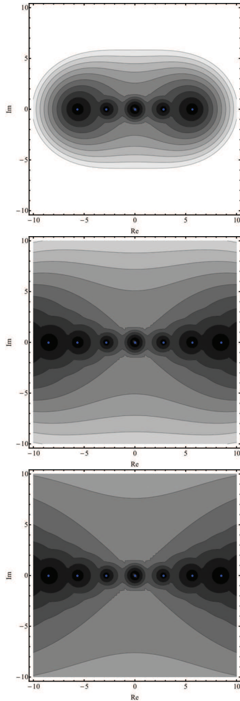
Figure 2. Eigenvalues (blue dots) and \varepsilon -pseudospectra of the truncated 4n \times 4n matrices A_n for n = 2 (top), n = 4 (middle), n = 6 (bottom) and \varepsilon = 1.5, 1.4, \dots, 0.6, 0.5 .
