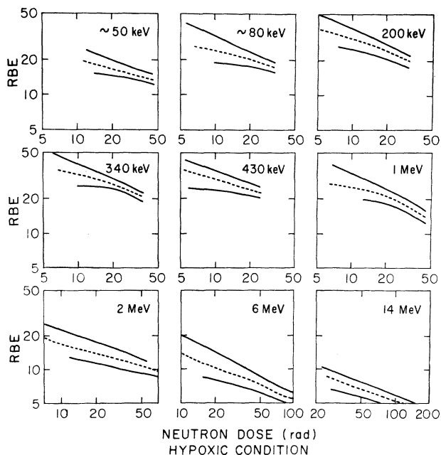
FIG. 8. Estimates (broken lines) of the dose-RBE dependence and the 95% confidence regions (solid lines) for various neutron energies under hyoxic conditions.
