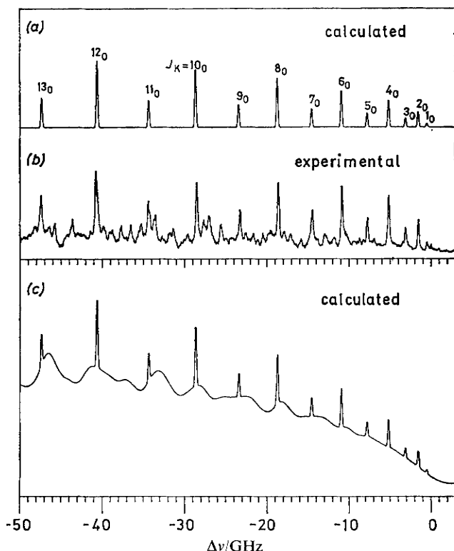
Fig. 4. (a) Calculated spectrum of a totally symmetric two-photon transition showing only K = 0 lines. (b) Corresponding part of the measured spectrum of the 14_0^+1_0^+ band shown in fig. 3(b). (c) Calculated spectrum showing sharp K = 0 lines (210 MHz f.w.h.m.) on top of a background caused by the many broadened (3 GHz f.w.h.m.) K \neq 0 lines [from ref. (17)].
