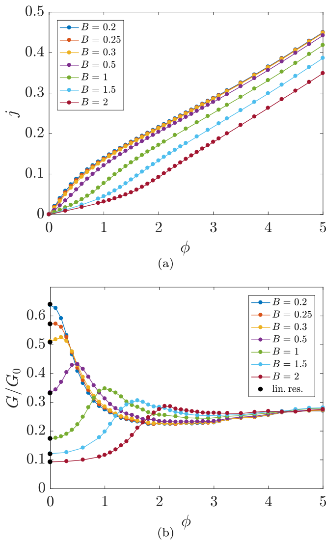
Figure 3. (a) Current–voltage characteristic j(\phi) and (b) differential conductance G(\phi) for different values of the magnetic field B . G is in units of G_0 = G(T = 0, \phi = 0) = e^2/(\pi\hbar) . Parameters are as in figure 1.
