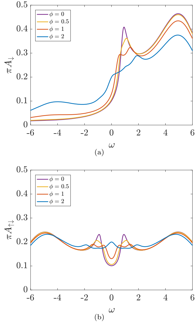
Figure 2. Nonequilibrium spin-resolved (a) and total (b) impurity spectral function for different values of the bias voltage \phi and fixed magnetic field B = \Gamma/(lg|\mu_B) ; T = 0.05\Gamma/k_B \approx T_K/2 . Note that \phi is in units of \Gamma/e . Here a larger value of U = 8\Gamma is chosen, in order to resolve the four-peak structure in A_{\uparrow\downarrow} .
