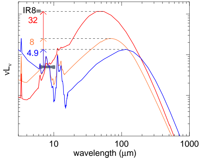
Fig. 11. Three SEDs from the Chary & Elbaz (2001) library normalized to the same L_{8\mu\text{m}} (using the IRAC passband centered on 8\mu\text{m} ). We present the SEDs 11, 58, and 95 for which IR8 = L_{\text{IR}}/L_{8\mu\text{m}} = 4.9, 8, \text{ and } 32 , respectively. The horizontal black solid segment shows the width of the IRAC2 channel centered on 8\mu\text{m} .
