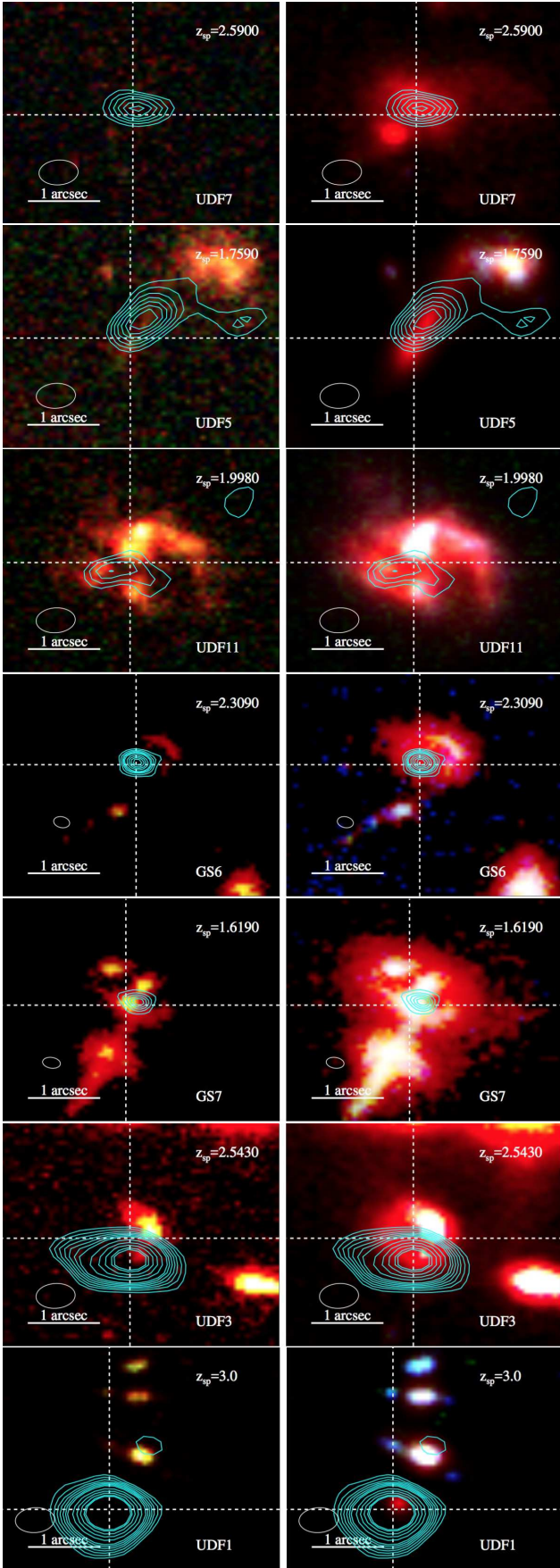
Fig. 7. As in Fig. 6 for the “starburst” galaxies with R_{SB} > 3 sorted by increasing R_{SB} from top to bottom. Contours as in Fig. 6.
