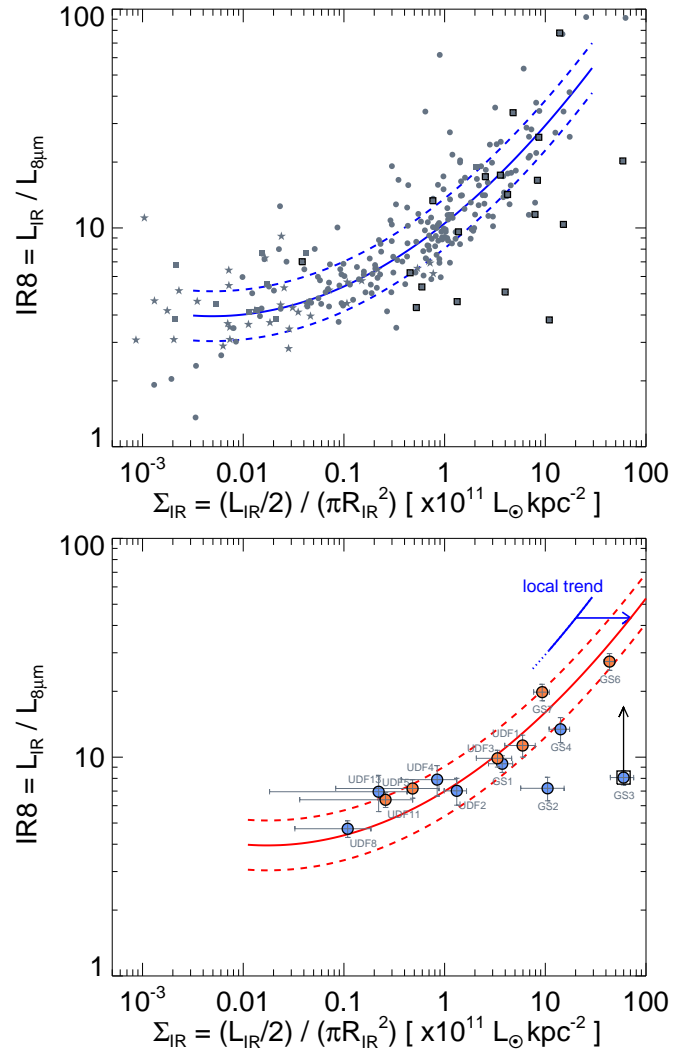
Fig. 12. Top: IR8 - \Sigma_{IR} relation for local galaxies. Gray filled dots: 293 galaxies with Herschel PACS 70 \mu\text{m} sizes ( R_{IR} = R_{70\mu\text{m}} ) from Díaz-Santos et al. (2017). Filled squares and stars: 11 and 39 galaxies with radio and MIR sizes from Elbaz et al. (2011). Galaxies with MIR spectral signatures of AGNs (identified by Díaz-Santos et al. 2017) are marked with bold squares. The solid blue line is a polynomial fit to the sliding median described by Eq. (7). The two dashed lines 30% above and below ( \pm 0.11 dex) encompass 68% of the galaxies. Bottom: position of the z \sim 2 ALMA sources on the IR8 - \Sigma_{IR} diagram. The solid and dashed red lines show the local relation shifted to the right by a factor 3.5 to account for the combined effects of the rise of the MS SFR with redshift and decrease of galaxy sizes with redshift. Blue and orange filled dots separate galaxies on or close to the MS ( R_{SB} \leq 3 ) from starbursts ( R_{SB} > 3 ). Only galaxies within 1.5 \leq z \leq 2.5 are shown here because of a large and uncertain extrapolation of L_8 from the observed 24 \mu\text{m} flux density for galaxies outside this redshift range. The black square on GS3 indicates that it is a power-law for which the contribution of the AGN has been corrected in a conservative way.
