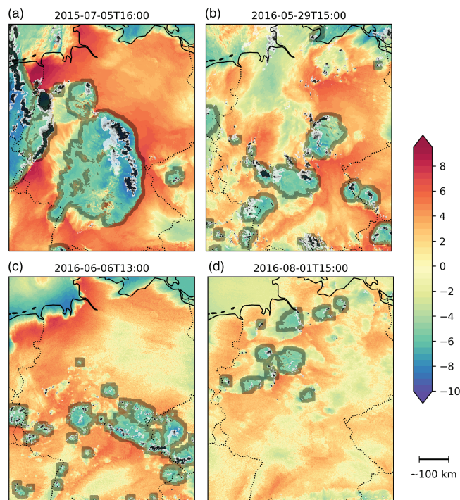
FIGURE 1 Example snapshots of buoyancy intensity ( \text{m}\cdot\text{s}^{-1} ; colour shading; Section 2.3.1), cold-pool boundary regions (grey shading) and precipitation intensity (white 1\text{ mm}\cdot\text{hr}^{-1} to black 20\text{ mm}\cdot\text{hr}^{-1} ) are displayed for each day from the 156 m grid size simulations. Dotted and solid black lines show country borders and coastlines respectively
