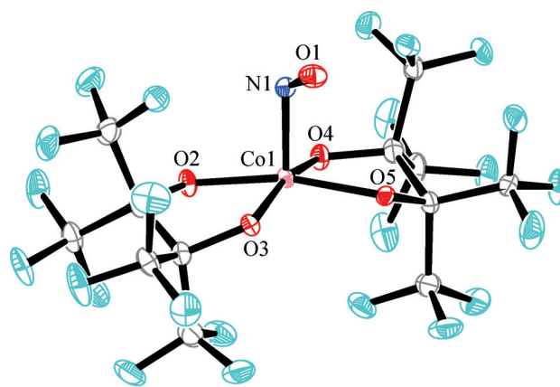
Figure 1. Ortep plot of the major disorder form (81%) of the anion of 1 , drawn at 70% ellipsoid probability. Distances in Å and angles in °: Co to: N1 1.793(2), O2 1.899(2), O3 1.904(3), O4 1.898(3), O5 1.901(2); N–O 1.185(3), Co–N–O 120.6(2).
