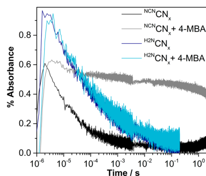
Figure 7. Transient decays probed at \lambda = 750 nm of ^{\text{NCN}}\text{CN}_x (1.2 \text{mg mL}^{-1} ) and ^{\text{H2N}}\text{CN}_x (1.2 \text{mg mL}^{-1} ) suspensions in aqueous \text{KP}_i solution (0.02 M, pH 4.5, 25 ^\circ\text{C} ) following \lambda = 355 nm excitation. Traces obtained following the addition of 10 mM 4-MBA are also shown.
