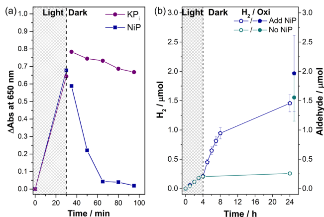
Figure 5. (a) Spectrophotometry of the appearance (during irradiation) and disappearance (upon addition of NiP in the dark) of photoexcited electrons in ^{\text{NCN}}\text{CN}_x at \lambda = 650 nm. A suspension with ^{\text{NCN}}\text{CN}_x (5 mg) and 4-MBA (30 \mu\text{mol} ) in \text{KP}_i (0.02 M, pH 4.5, 3 mL) was irradiated (AM 1.5G) for 30 min, followed by addition of NiP (50 nmol, 400 \mu\text{L} ) or \text{KP}_i (400 \mu\text{L} ). (b) Two photoreactors were prepared with ^{\text{NCN}}\text{CN}_x (5 mg) and 4-MBA (30 \mu\text{mol} ) in the absence of NiP in an aqueous \text{KP}_i solution (0.02 M, pH 4.5, 3 mL) and irradiated with 1 sun irradiation (AM 1.5G, 25 ^\circ\text{C} ). Both of these photoreactors were taken into the dark after 4 h of irradiation, while NiP (50 nmol) was added to one of them. The pair of hollow and filled symbols of the same shape and color corresponds to \text{H}_2 and aldehyde production, respectively, under the specified reaction conditions.
