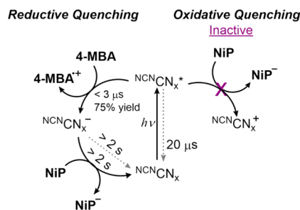
Figure 6. Summary of mechanism and kinetic rates from TAS measurements with suspensions of ^{\text{NCN}}\text{CN}_x (1–5 \text{mg mL}^{-1} ), NiP (up to 24 \mu\text{M} ), and 4-MBA (10 mM) in an aqueous \text{KP}_i solution (0.02 M, pH 4.5, 25 ^\circ\text{C} ). Representative lifetimes, calculated using 3 \mu\text{s} as the initial time, are indicated near reaction arrows. Recombination reactions are indicated by dashed gray arrows.
