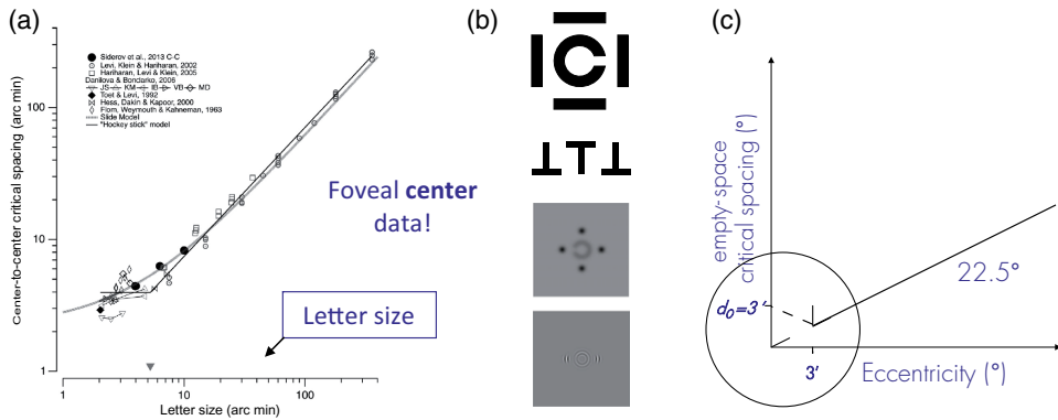
Figure 6. (A) Coates and Levi’s (2014) Figure 4, annotated, illustrating their “hockey stick model” that describes the dependence of centre-to-centre critical spacing on target size. The filled circles show Siderov et al.’s (2013) data for Sloan letters surrounded by bars. Note that the slope is \approx 1.0 , that is, an increase of letter size leads to an increase of centre-to-centre critical spacing by the same amount. The figure is annotated to emphasize that the abscissa is different from the previous figures and no eccentric data are shown. (B) A wide range of stimuli underlie the data shown in that figure, among them (top) the classical arrangement of Flom et al. (1963) or Toet and Levi’s (1992) Ts (reproduced from Strasburger et al., 2011, Figure 19B, and A. Toet, personal communication, 19 Apr 2020, respectively) and also (bottom) various Gaussian and Gabor targets (Hariharan et al., 2005, from Figure 1 and Figure 2; blur intentional). (C) Possible shapes of Bouma’s law in the visual field’s very centre (with a slope of 0.5 = 22.5^\circ ) that would be compatible with the hockey stick model.
