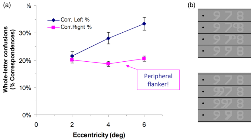
Figure 16. (A) Reverse Asymmetry in a Crowding Task Reported in Strasburger and Malania (2013, Figure 8A; modified). Confusions with the more central, but not the more peripheral, flanker depend on eccentricity. (B) Cartoon, as a memory aid for the mechanisms: (top) a peripheral letter part moving inward; (bottom) the more central flanker moving outward. Note that the cartoon does not quite capture the effect of features because these are a much more general concept than pattern parts.
