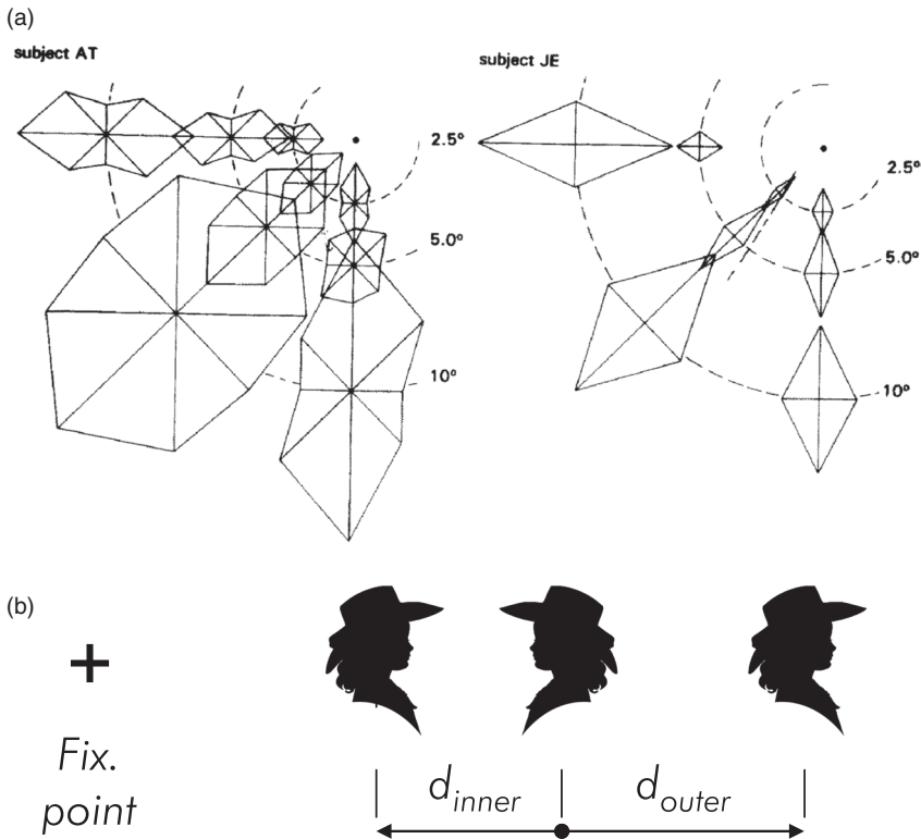
Figure 13. Crowding Asymmetries. (A) Radially elongated interaction fields for two subjects from Toet and Levi (1992, Figure 6), showing the well-known radial-tangential anisotropy where flankers on a radius from the visual field centre exert more influence than those arranged tangentially. (B) The inner-outer asymmetry, first studied by Mackworth (1965), refers to a different critical distance of the more peripheral versus the more central flanker. It will lead to asymmetrically elongated interaction fields.
