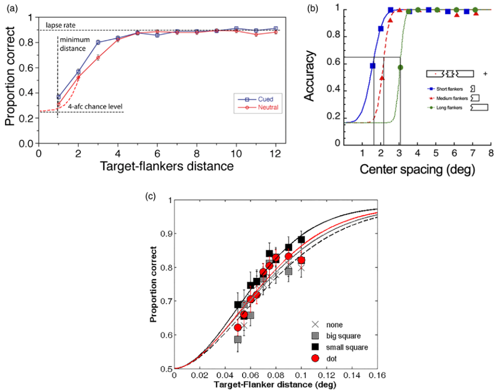
Figure 11. Examples of Psychometric Functions Versus Flanker Distance. (A) For letter-T recognition (the red line; disregard the blue line; eccentricity 9^\circ ; flanker distance in multiples of 0.9^\circ ). Modified from Yeshurun and Rashal (2010, Figure 5). (B) Example from Rosen et al. (2014, Figure 9A) with novel patterns that allow widening the flankers; the inset shows the stimulus and the legend; eccentricity 12^\circ . (C) Another recent example used for quantifying spatial attention (Albonico et al., 2018, Figure 4). The four conditions refer to the kinds of attentional cue used in the study; only “none,” that is, the no-cue condition, is relevant here. Foveal view.
