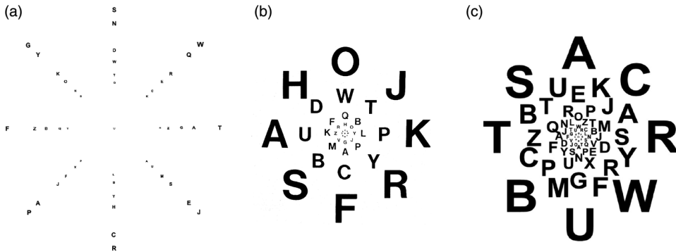
Figure 9. Figures 2, 3, and 4 in Anstis (1974), Illustrating Cortical Magnification. (A) Letter sizes are according to an estimate of the cortical-magnification factor (left). (B) Letters are shown at a 10-fold increased size (middle). (C) Letter sizes are the same, but more letters are added, to increase crowding (right).
