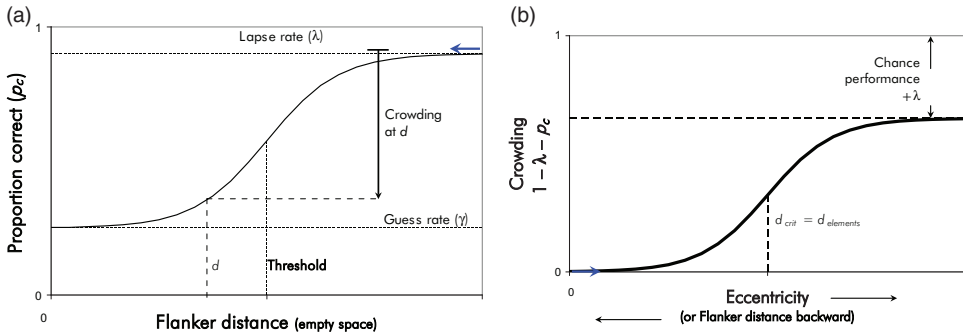
Figure 12. Schematic Depiction of Crowding as Defined Standardly, That Is, as the Impairment of Recognition Performance by the Presence of Flankers. (A) Psychometric function for proportion-correct performance in a crowding task, as in Figure 11. The effect of crowding, at some flanker distance d , is seen as the downward arrow on the right, starting from best performance ( 1-\lambda ). (B) Crowding as in Part A, but now as a function of eccentricity. Part B results from Part A by mirroring the psychometric-function graph both horizontally and vertically and rescaling the y axis appropriately. The blue arrow serves as a graphical aid.
