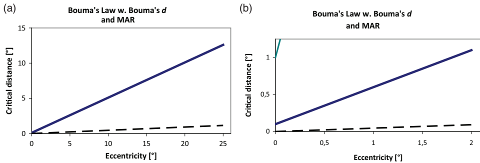
Figure 10. Bouma's Law (Continuous Line, as in Figure 4A), Compared With the Increase of the MAR With Eccentricity (Dashed Line; Data From Anstis, 1974, Figure 1). Critical distance and MAR are measured in the same units (visual angle) so that these can be directly compared. The graph is shown at two scales (Part A vs. B, as in Figure 4 vs. 5 above), to illustrate that, at a large scale, the slope difference matters most, whereas at a small scale, the intercept difference is more important. Part B of the figure has an additional line starting at 1° (dark green) that shows a hypothetical M -scaling function scaled the same as the acuity function in the graph (see the following text). MAR = minimal angle of resolution.
