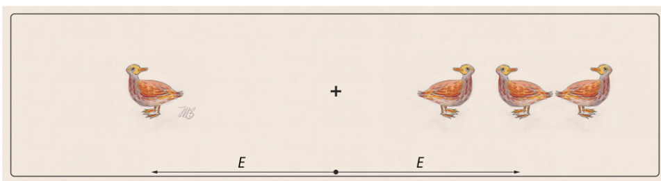
Figure 1. Simple Demonstration of Crowding. When fixating at the cross, the orientation for the duck on the left is seen but not that for the middle one on the right, even though the images are of the same size and at the same eccentricity. The phenomenon depends predominantly on eccentricity and pattern spacing and is mostly independent of target size. Duck painting by Ilse Maria Baumgart, Munich, 2019.
