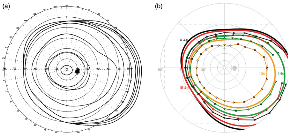
Figure 7. (A) The visual field, as drawn by Traquair (1938, Figure 1) in his classical book, based on the data by Rönne (1915). The outermost contour was obtained with a somewhat larger stimulus of 160 mm diameter, presented at 1 m viewing distance, that is, of 9^\circ size. (B) A recent visual field map obtained with reaction time-corrected, semiautomated kinetic perimetry (Vonthein et al., 2007, Figure 3A).
