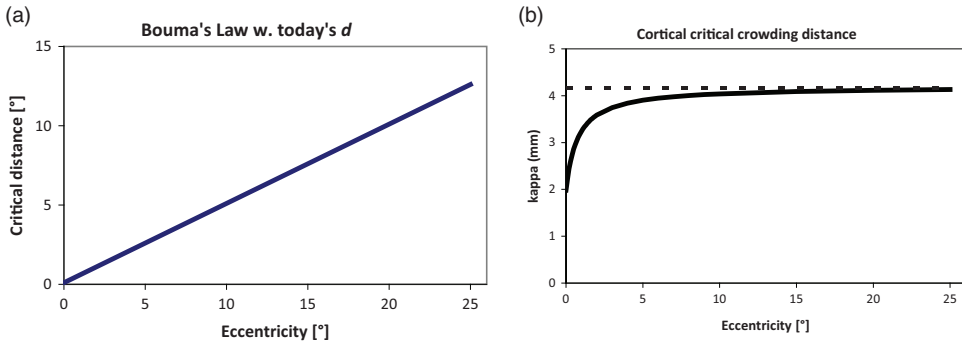
Figure 17. (A) Bouma's law in the visual field and (B) its cortical equivalent, that is, how it translates to the cortical map in a primary visual area (Strasburger, 2019, Figure 8; see there for the specific parameters chosen for the estimation and note that kappa depends upon these).
