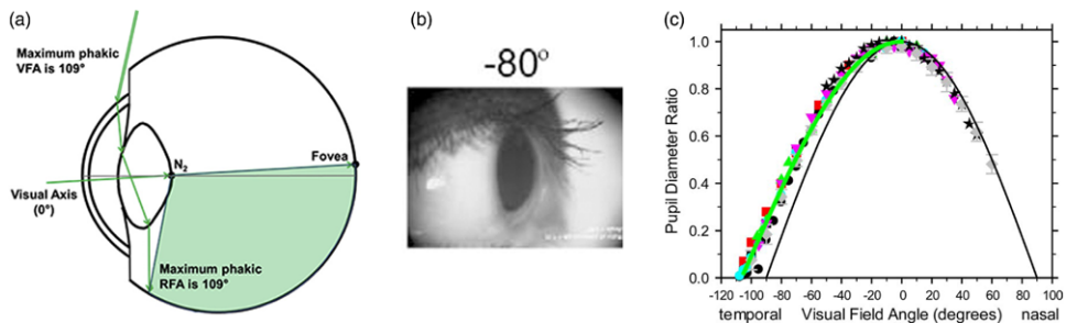
Figure 8. (A) Ray-trace model of how light enters the eye at the maximum angle for a 5-mm pupil (Holladay & Simpson, 2017, Figure 3A). (B) Pupil as seen from an angle of 80° on the temporal side (Mathur et al., 2013, Figure 5). (C) Aspect ratio of the pupil's shape as seen by an observer under different horizontal angles, with data from eight different studies in the literature (coloured symbols; Mathur et al., 2013, Figure 1). VFA = visual field angle; RFA = retinal field angle.
