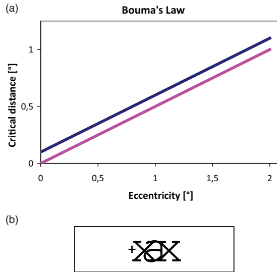
Figure 5. (A) Comparison of Bouma's law with critical distance defined as empty space (pink) versus centre-to-centre (blue). (B) A degenerated stimulus configuration with overlapping flankers that would result from an incorrect statement of Bouma's law at small eccentricity.
